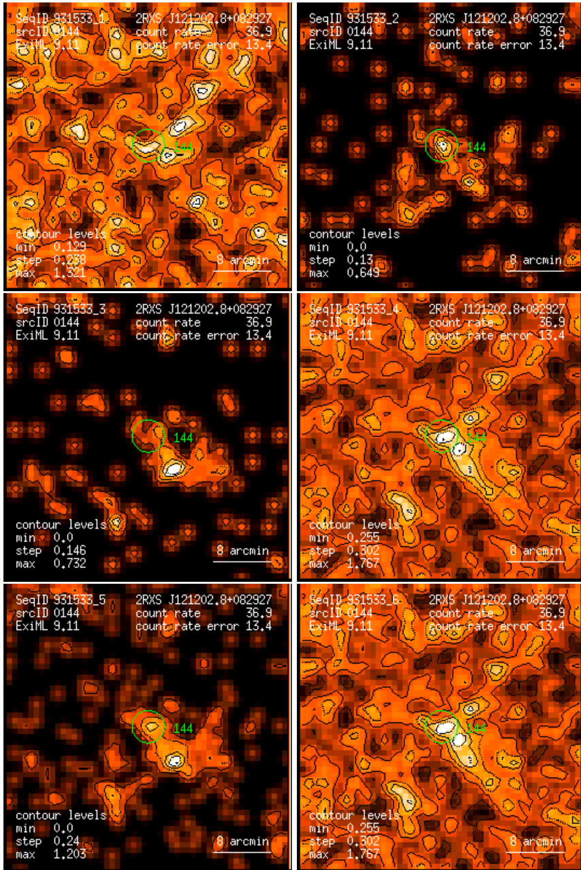
Figure 144: RASS 931533: detection 0144: band rate images, Gaussian filter: (1) PSPC channels 11 – 41, (2) 52 – 90, (3) 91 – 201, (4) 11 – 235, (5) 52 – 201, (6) 11 – 201. Broad band rates in counts/ks. Band rate contour levels in counts/ks/arcmin 2 .
