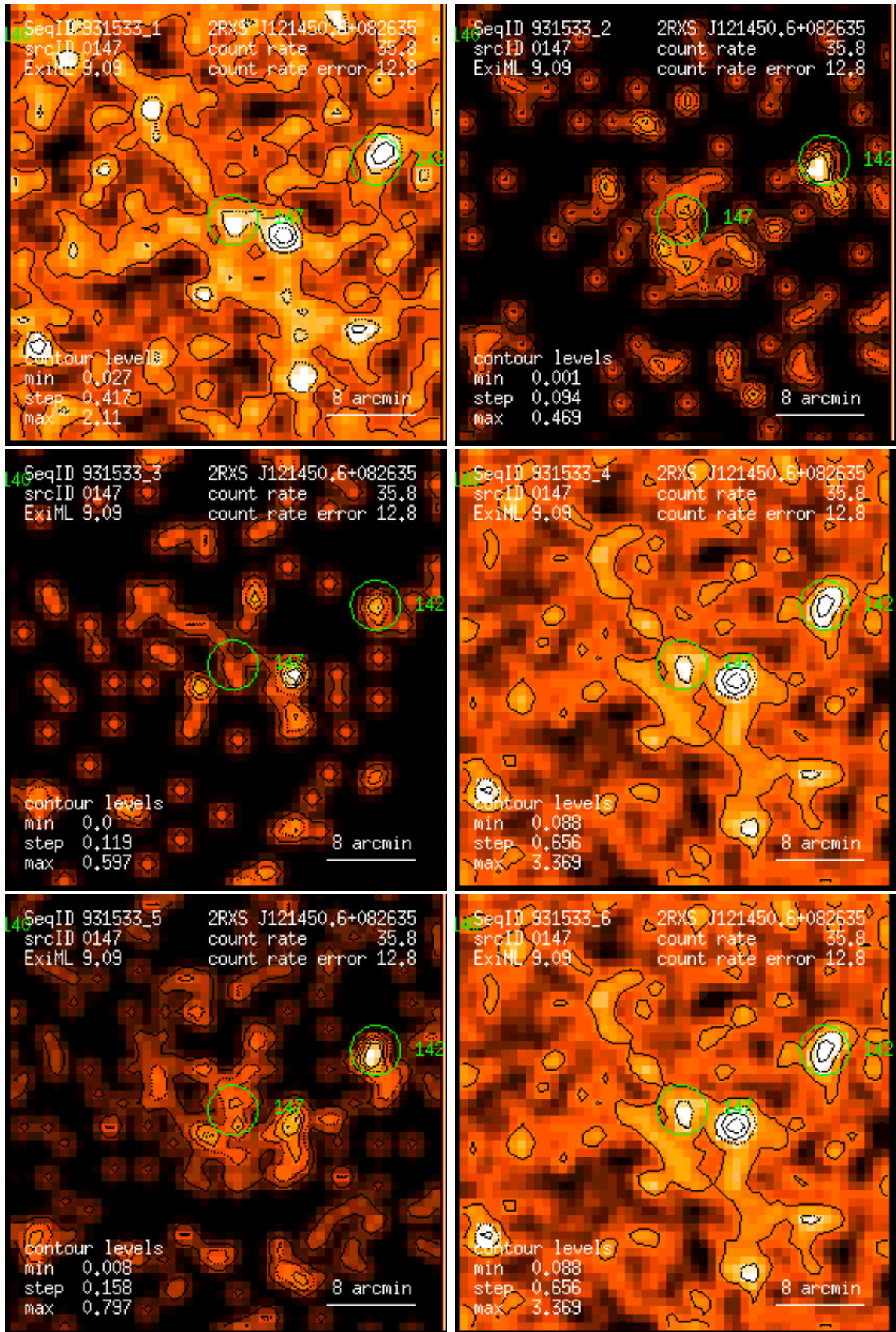
Figure 147: RASS 931533: detection 0147: band rate images, Gaussian filter: (1) PSPC channels 11 – 41, (2) 52 – 90, (3) 91 – 201, (4) 11 – 235, (5) 52 – 201, (6) 11 – 201. Broad band rates in counts/ks. Band rate contour levels in counts/ks/arcmin 2 .
