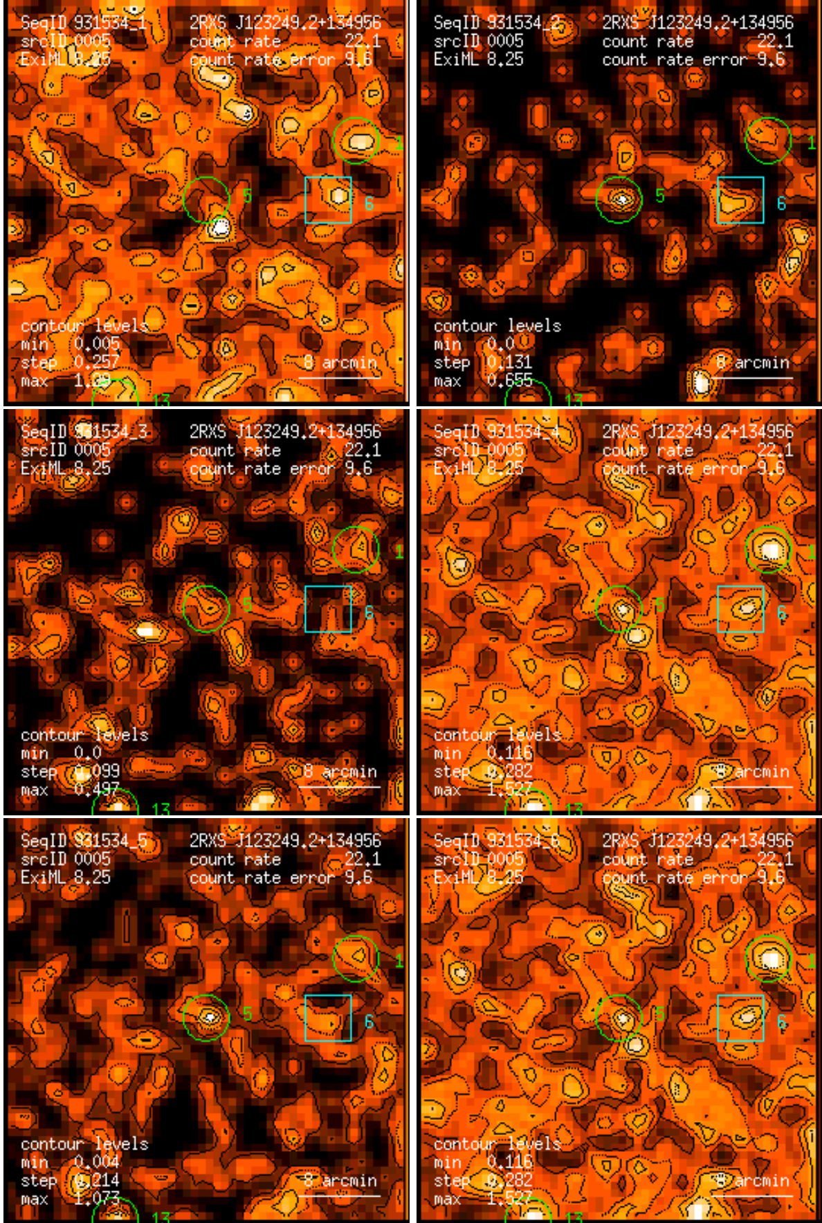
Figure 5: RASS 931534: detection 0005: band rate images, Gaussian filter: (1) PSPC channels 11 – 41, (2) 52 – 90, (3) 91 – 201, (4) 11 – 235, (5) 52 – 201, (6) 11 – 201. Broad band rates in counts/ks. Band rate contour levels in counts/ks/arcmin 2 .
