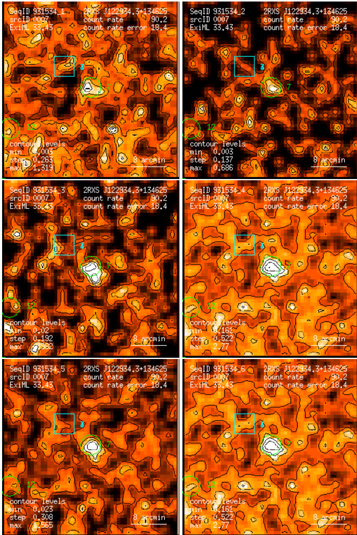
Figure 7: RASS 931534: detection 0007: band rate images, Gaussian filter: (1) PSPC channels 11 – 41, (2) 52 – 90, (3) 91 – 201, (4) 11 – 235, (5) 52 – 201, (6) 11 – 201. Broad band rates in counts/ks. Band rate contour levels in counts/ks/arcmin 2 .
