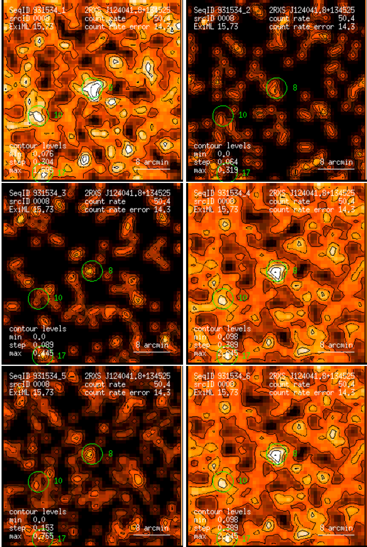
Figure 8: RASS 931534: detection 0008: band rate images, Gaussian filter: (1) PSPC channels 11 – 41, (2) 52 – 90, (3) 91 – 201, (4) 11 – 235, (5) 52 – 201, (6) 11 – 201. Broad band rates in counts/ks. Band rate contour levels in counts/ks/arcmin 2 .
