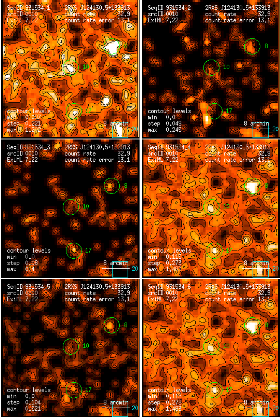
Figure 10: RASS 931534: detection 0010: band rate images, Gaussian filter: (1) PSPC channels 11 – 41, (2) 52 – 90, (3) 91 – 201, (4) 11 – 235, (5) 52 – 201, (6) 11 – 201. Broad band rates in counts/ks. Band rate contour levels in counts/ks/arcmin 2 .
