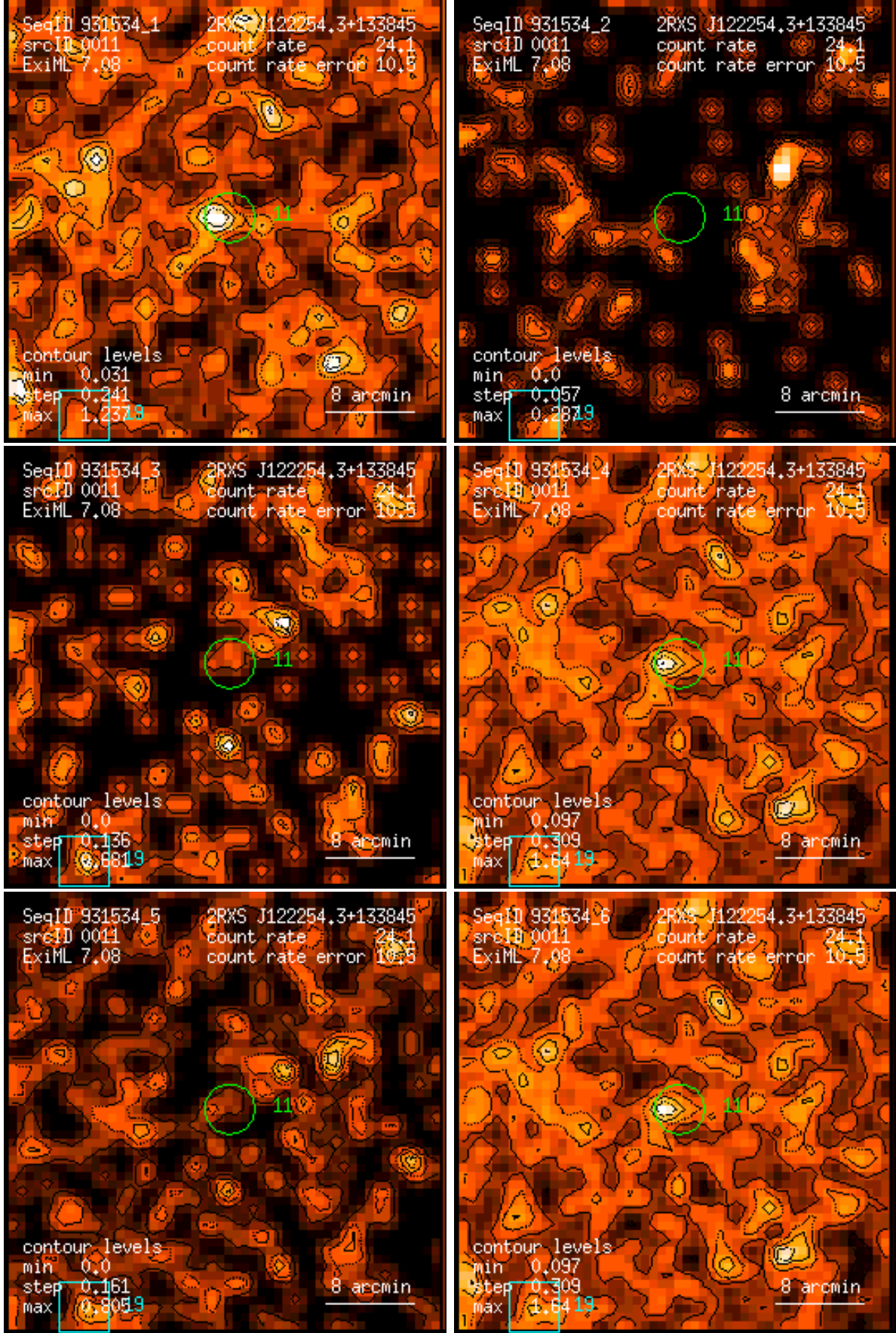
Figure 11: RASS 931534: detection 0011: band rate images, Gaussian filter: (1) PSPC channels 11 – 41, (2) 52 – 90, (3) 91 – 201, (4) 11 – 235, (5) 52 – 201, (6) 11 – 201. Broad band rates in counts/ks. Band rate contour levels in counts/ks/arcmin 2 .
