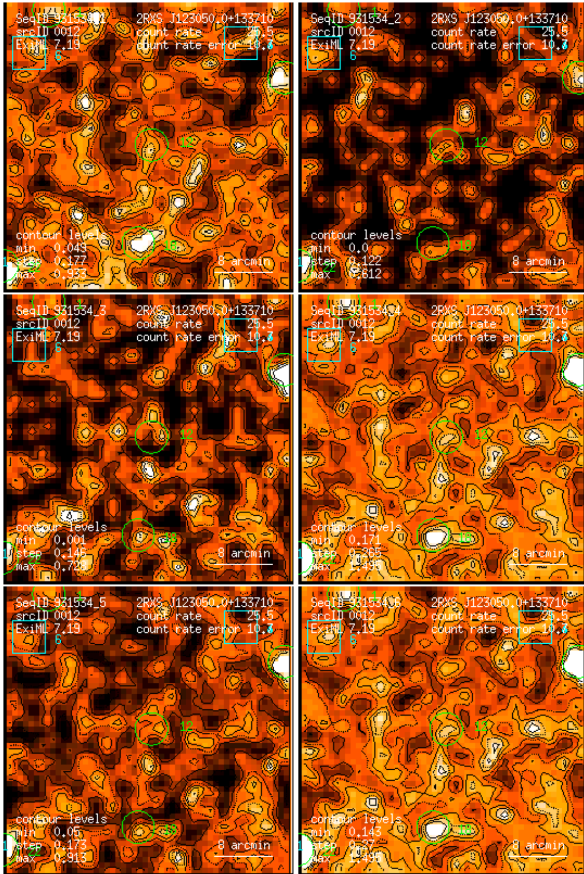
Figure 12: RASS 931534: detection 0012: band rate images, Gaussian filter: (1) PSPC channels 11 – 41, (2) 52 – 90, (3) 91 – 201, (4) 11 – 235, (5) 52 – 201, (6) 11 – 201. Broad band rates in counts/ks. Band rate contour levels in counts/ks/arcmin 2 .
