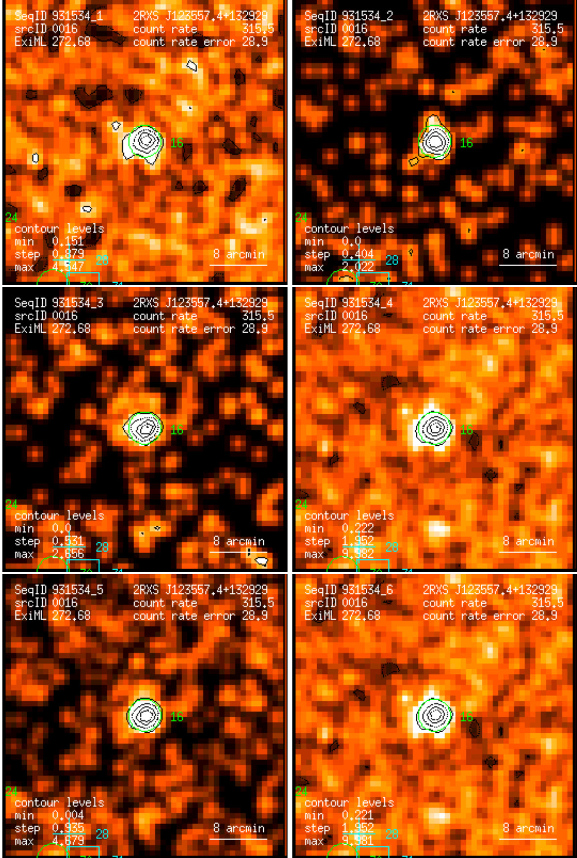
Figure 16: RASS 931534: detection 0016: band rate images, Gaussian filter: (1) PSPC channels 11 – 41, (2) 52 – 90, (3) 91 – 201, (4) 11 – 235, (5) 52 – 201, (6) 11 – 201. Broad band rates in counts/ks. Band rate contour levels in counts/ks/arcmin 2 .
