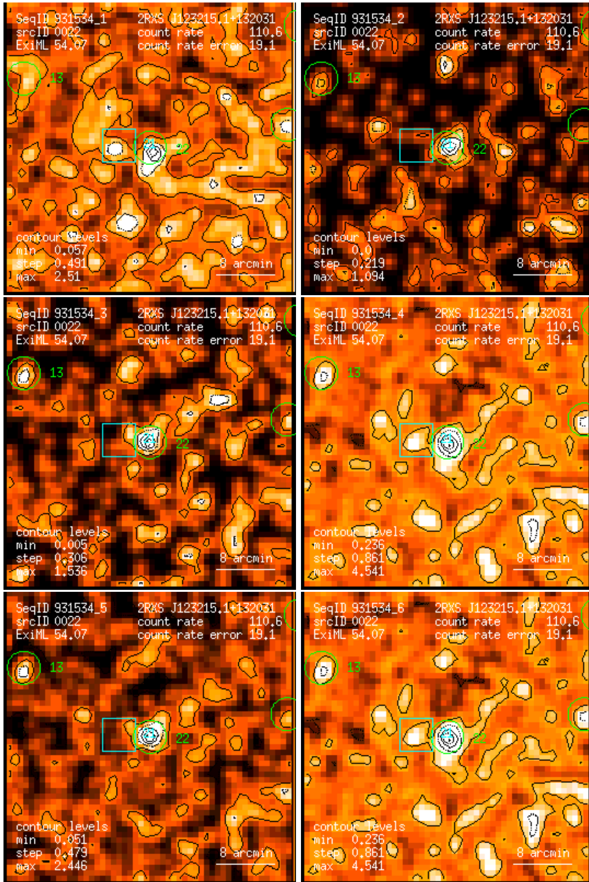
Figure 22: RASS 931534: detection 0022: band rate images, Gaussian filter: (1) PSPC channels 11 – 41, (2) 52 – 90, (3) 91 – 201, (4) 11 – 235, (5) 52 – 201, (6) 11 – 201. Broad band rates in counts/ks. Band rate contour levels in counts/ks/arcmin 2 .
