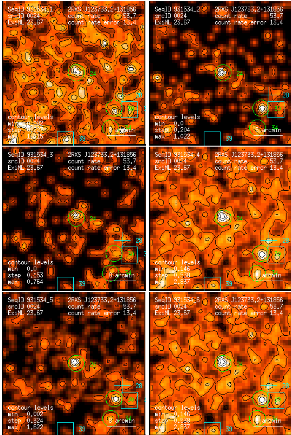
Figure 24: RASS 931534: detection 0024: band rate images, Gaussian filter: (1) PSPC channels 11 – 41, (2) 52 – 90, (3) 91 – 201, (4) 11 – 235, (5) 52 – 201, (6) 11 – 201. Broad band rates in counts/ks. Band rate contour levels in counts/ks/arcmin 2 .
