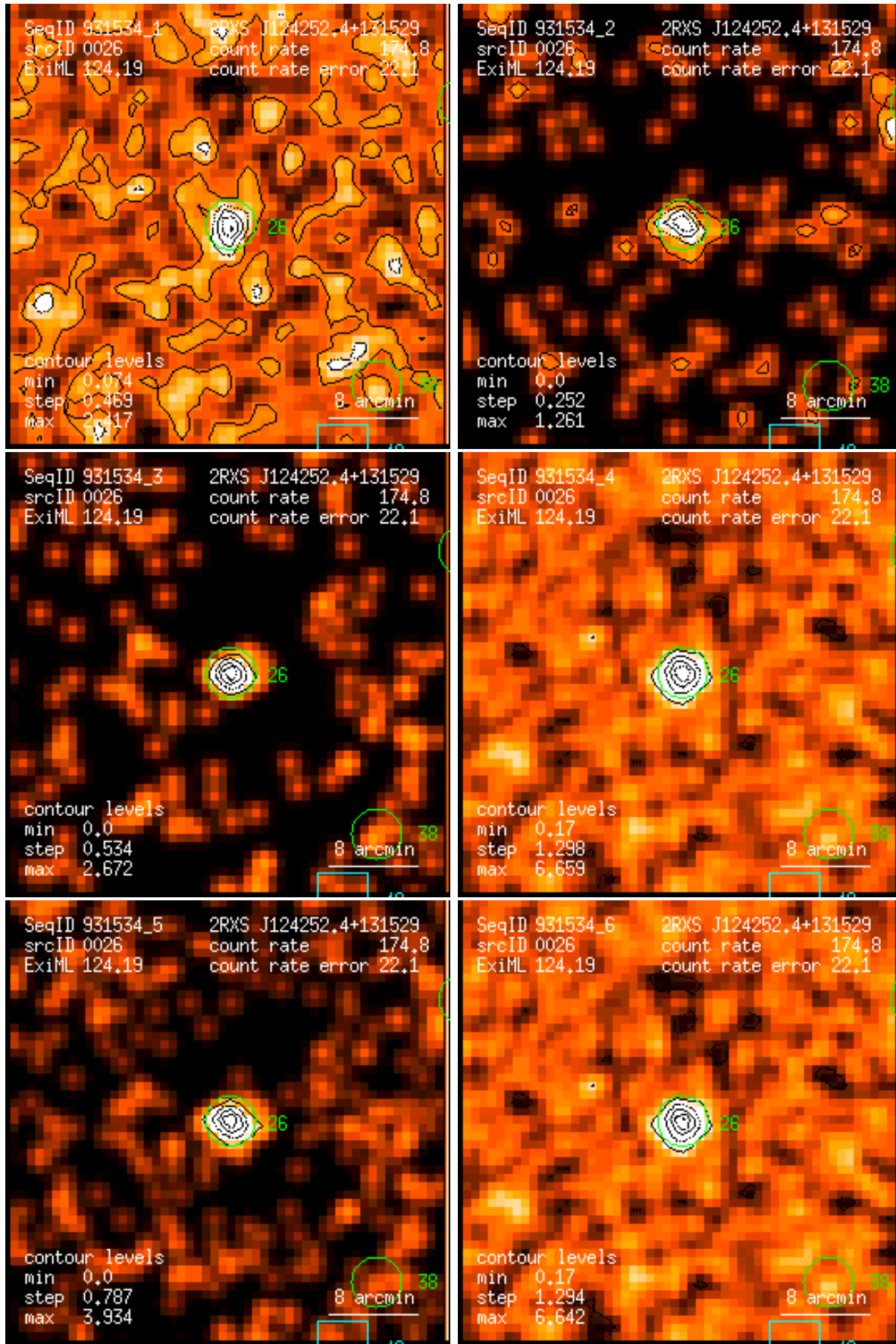
Figure 26: RASS 931534: detection 0026: band rate images, Gaussian filter: (1) PSPC channels 11 – 41, (2) 52 – 90, (3) 91 – 201, (4) 11 – 235, (5) 52 – 201, (6) 11 – 201. Broad band rates in counts/ks. Band rate contour levels in counts/ks/arcmin 2 .
