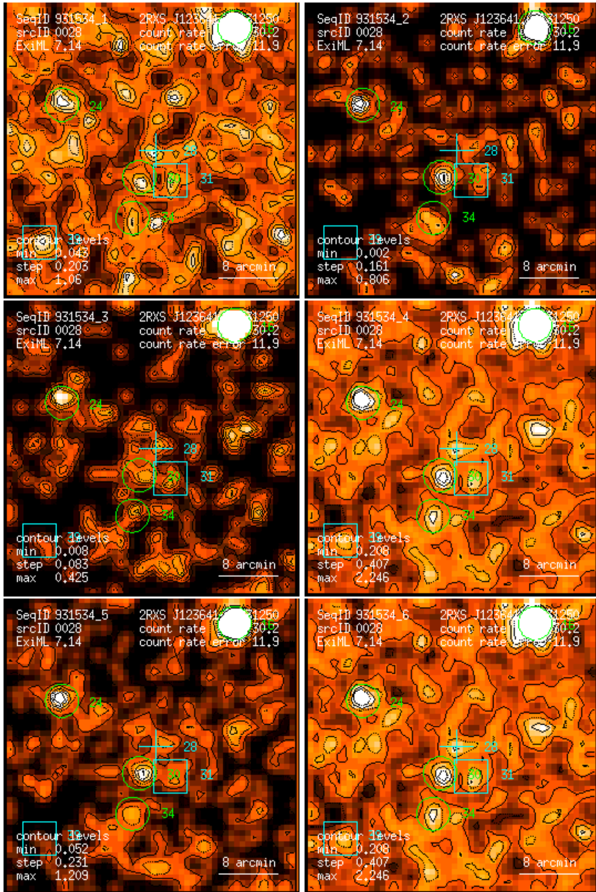
Figure 28: RASS 931534: detection 0028: band rate images, Gaussian filter: (1) PSPC channels 11 – 41, (2) 52 – 90, (3) 91 – 201, (4) 11 – 235, (5) 52 – 201, (6) 11 – 201. Broad band rates in counts/ks. Band rate contour levels in counts/ks/arcmin 2 .
