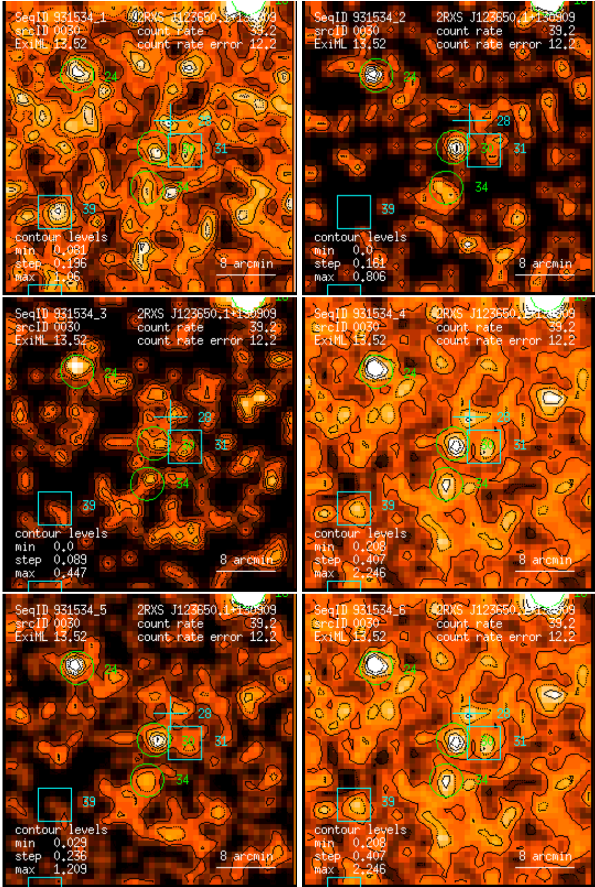
Figure 30: RASS 931534: detection 0030: band rate images, Gaussian filter: (1) PSPC channels 11 – 41, (2) 52 – 90, (3) 91 – 201, (4) 11 – 235, (5) 52 – 201, (6) 11 – 201. Broad band rates in counts/ks. Band rate contour levels in counts/ks/arcmin 2 .
