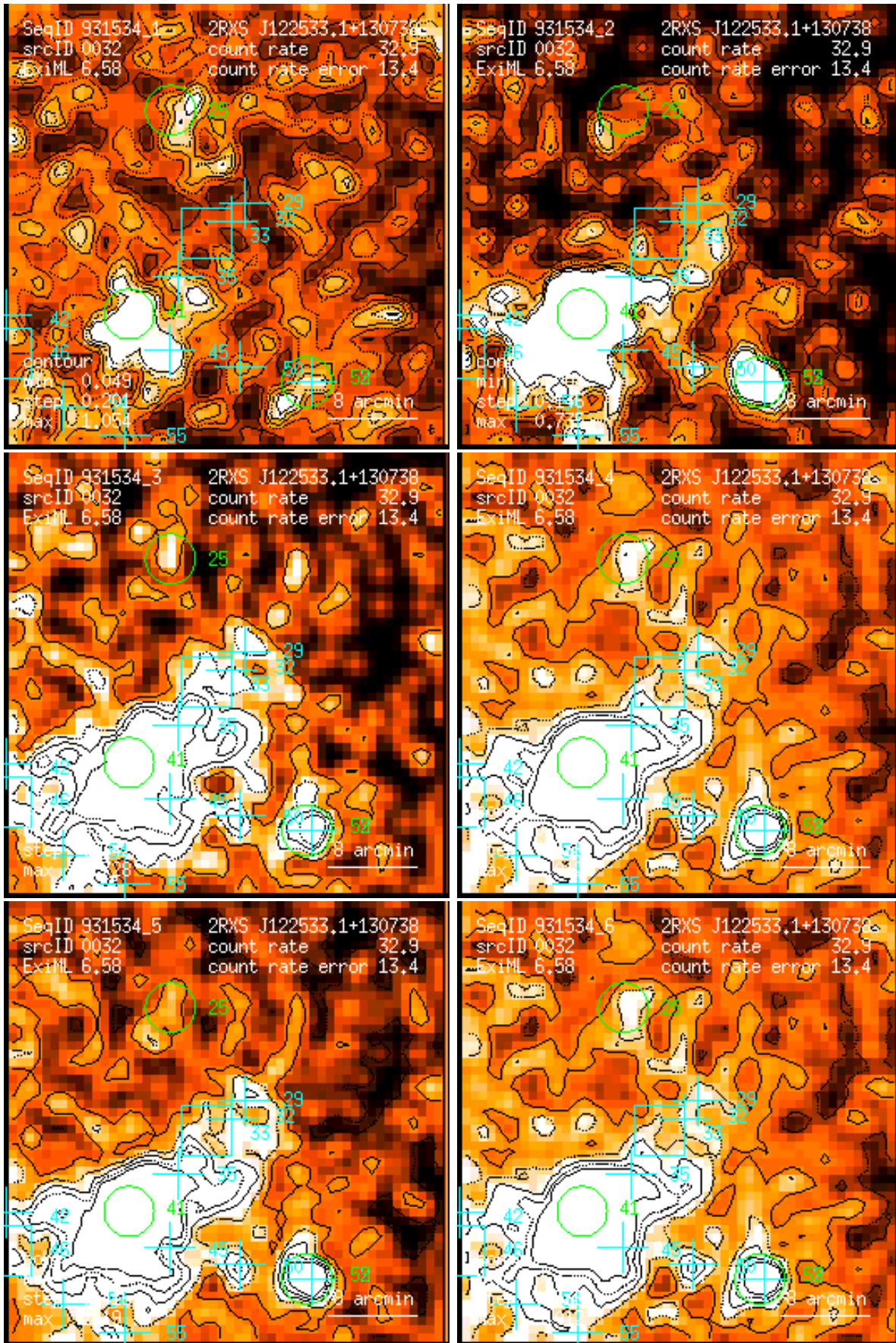
Figure 32: RASS 931534: detection 0032: band rate images, Gaussian filter: (1) PSPC channels 11 – 41, (2) 52 – 90, (3) 91 – 201, (4) 11 – 235, (5) 52 – 201, (6) 11 – 201. Broad band rates in counts/ks. Band rate contour levels in counts/ks/arcmin 2 .
