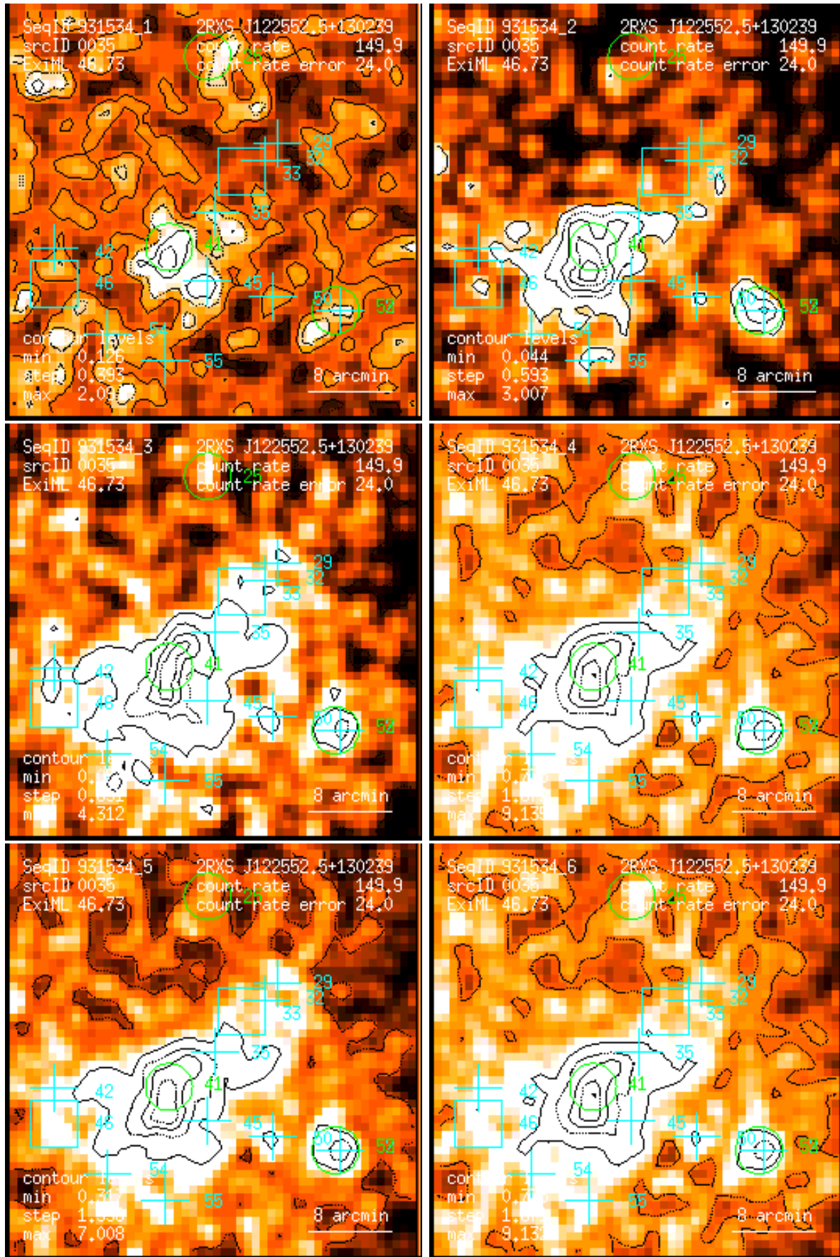
Figure 35: RASS 931534: detection 0035: band rate images, Gaussian filter: (1) PSPC channels 11 – 41, (2) 52 – 90, (3) 91 – 201, (4) 11 – 235, (5) 52 – 201, (6) 11 – 201. Broad band rates in counts/ks. Band rate contour levels in counts/ks/arcmin 2 .
