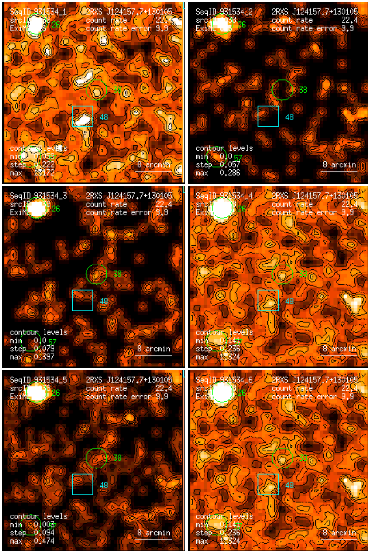
Figure 38: RASS 931534: detection 0038: band rate images, Gaussian filter: (1) PSPC channels 11 – 41, (2) 52 – 90, (3) 91 – 201, (4) 11 – 235, (5) 52 – 201, (6) 11 – 201. Broad band rates in counts/ks. Band rate contour levels in counts/ks/arcmin 2 .
