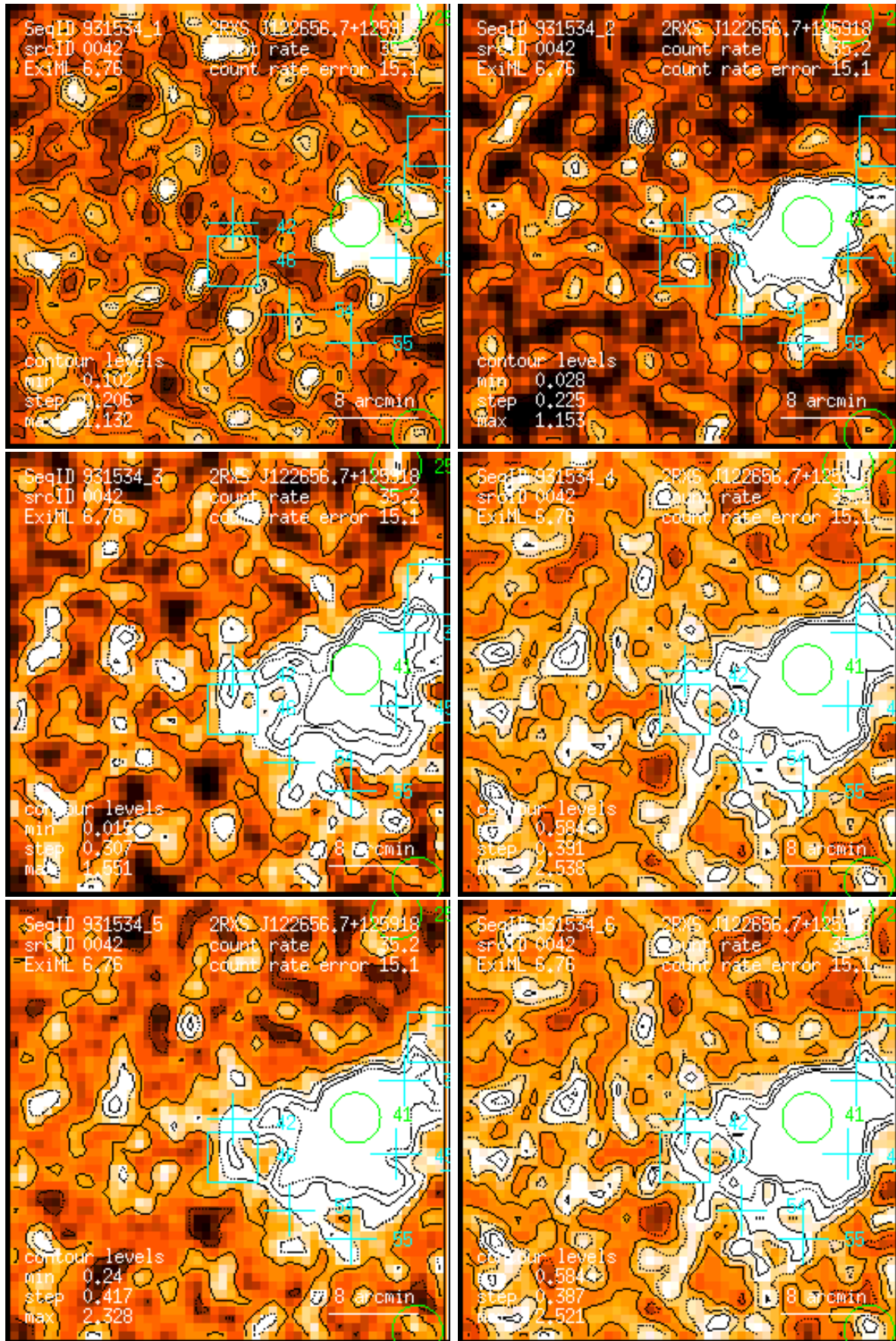
Figure 42: RASS 931534: detection 0042: band rate images, Gaussian filter: (1) PSPC channels 11 – 41, (2) 52 – 90, (3) 91 – 201, (4) 11 – 235, (5) 52 – 201, (6) 11 – 201. Broad band rates in counts/ks. Band rate contour levels in counts/ks/arcmin 2 .
