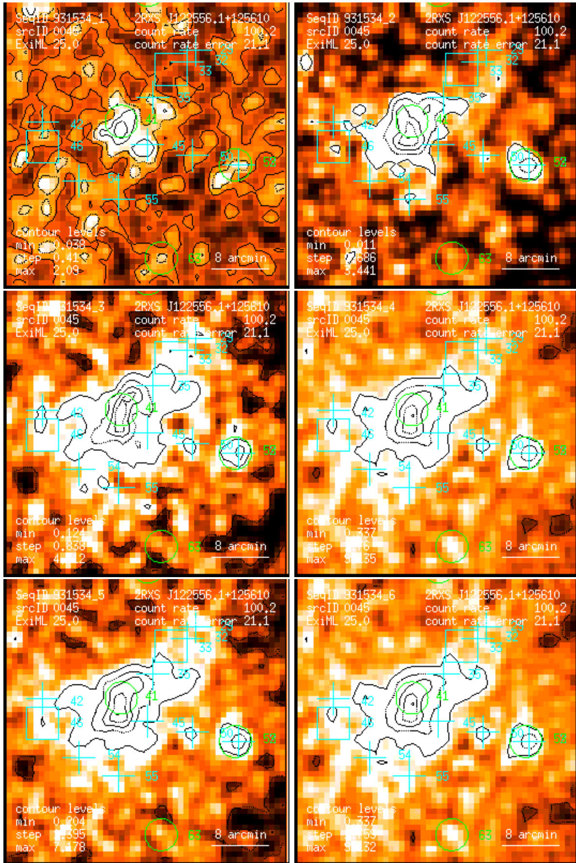
Figure 45: RASS 931534: detection 0045: band rate images, Gaussian filter: (1) PSPC channels 11 – 41, (2) 52 – 90, (3) 91 – 201, (4) 11 – 235, (5) 52 – 201, (6) 11 – 201. Broad band rates in counts/ks. Band rate contour levels in counts/ks/arcmin 2 .
