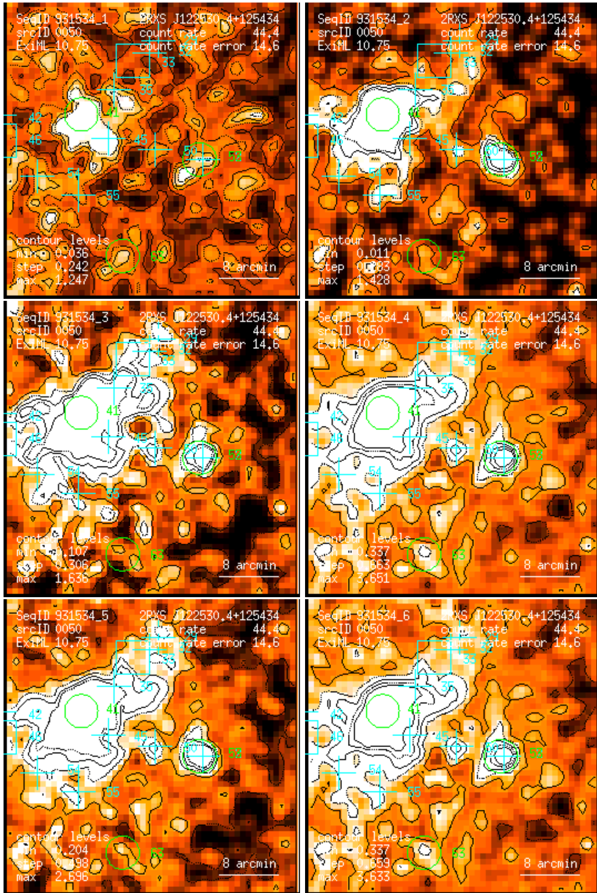
Figure 50: RASS 931534: detection 0050: band rate images, Gaussian filter: (1) PSPC channels 11 – 41, (2) 52 – 90, (3) 91 – 201, (4) 11 – 235, (5) 52 – 201, (6) 11 – 201. Broad band rates in counts/ks. Band rate contour levels in counts/ks/arcmin 2 .
