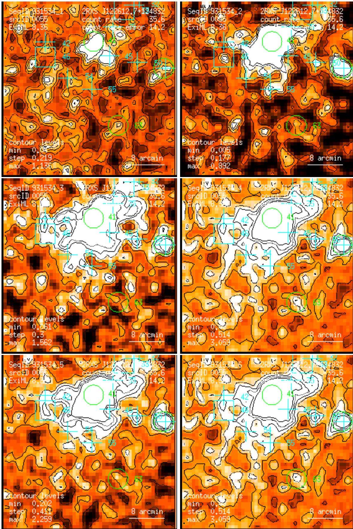
Figure 55: RASS 931534: detection 0055: band rate images, Gaussian filter: (1) PSPC channels 11 – 41, (2) 52 – 90, (3) 91 – 201, (4) 11 – 235, (5) 52 – 201, (6) 11 – 201. Broad band rates in counts/ks. Band rate contour levels in counts/ks/arcmin 2 .
