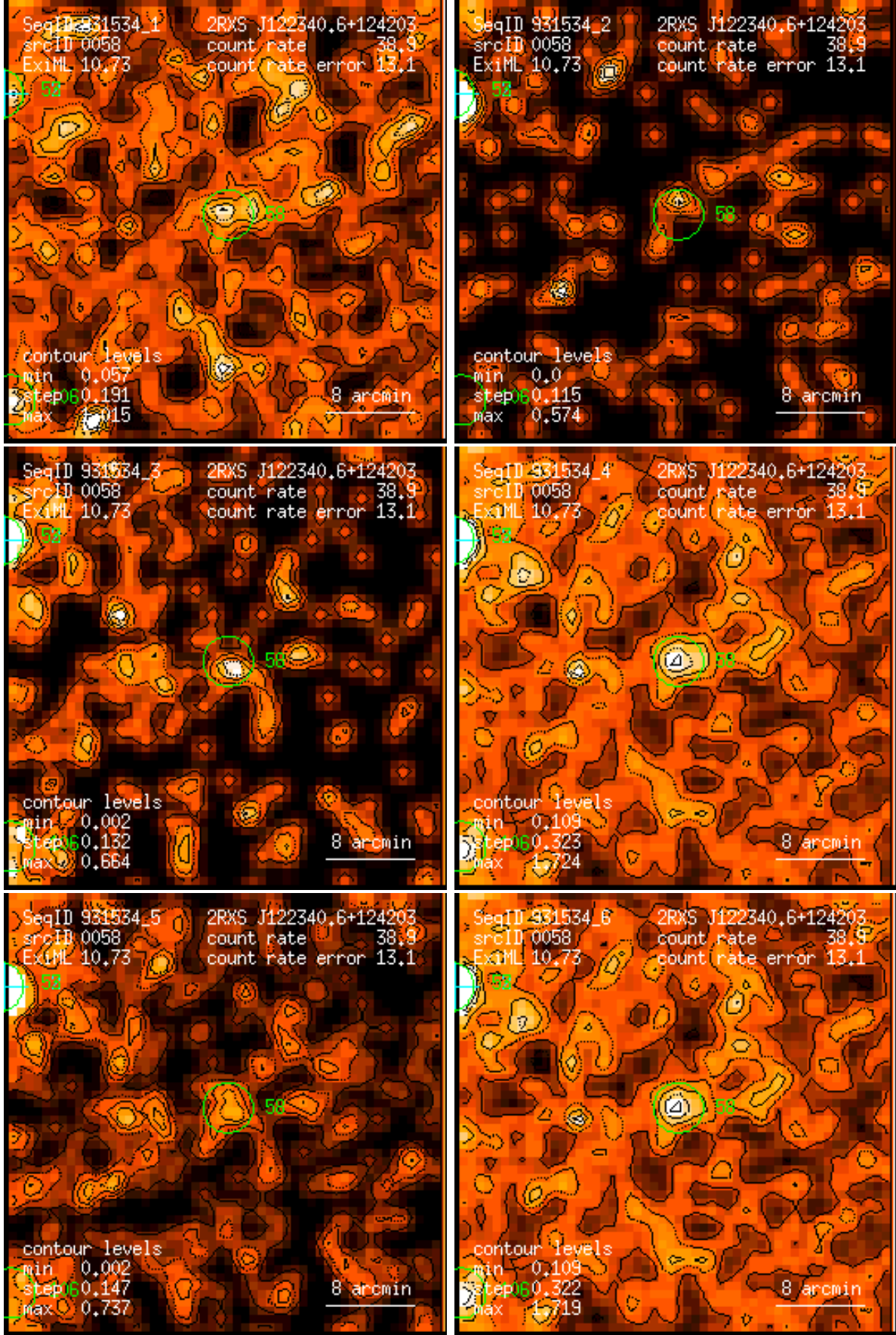
Figure 58: RASS 931534: detection 0058: band rate images, Gaussian filter: (1) PSPC channels 11 – 41, (2) 52 – 90, (3) 91 – 201, (4) 11 – 235, (5) 52 – 201, (6) 11 – 201. Broad band rates in counts/ks. Band rate contour levels in counts/ks/arcmin 2 .
