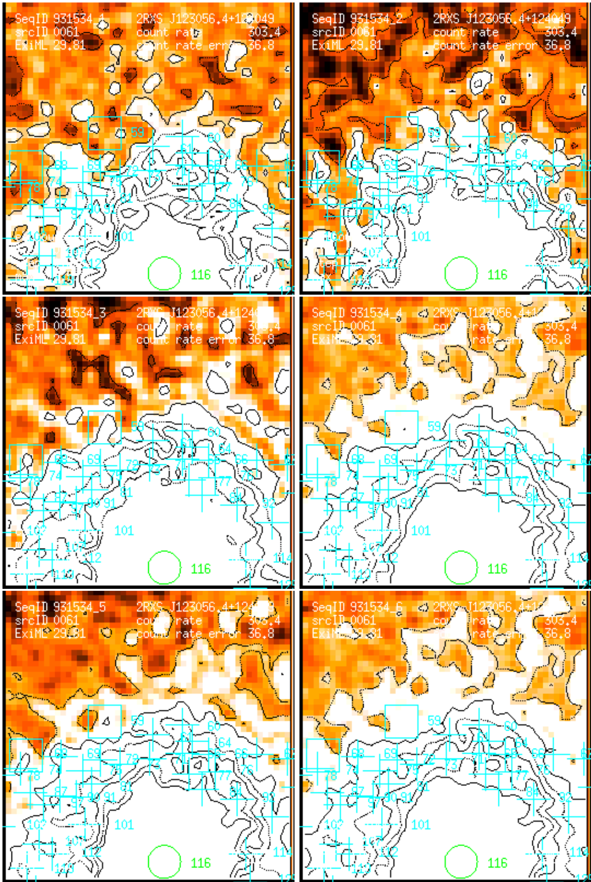
Figure 61: RASS 931534: detection 0061: band rate images, Gaussian filter: (1) PSPC channels 11 – 41, (2) 52 – 90, (3) 91 – 201, (4) 11 – 235, (5) 52 – 201, (6) 11 – 201. Broad band rates in counts/ks. Band rate contour levels in counts/ks/arcmin 2 .
