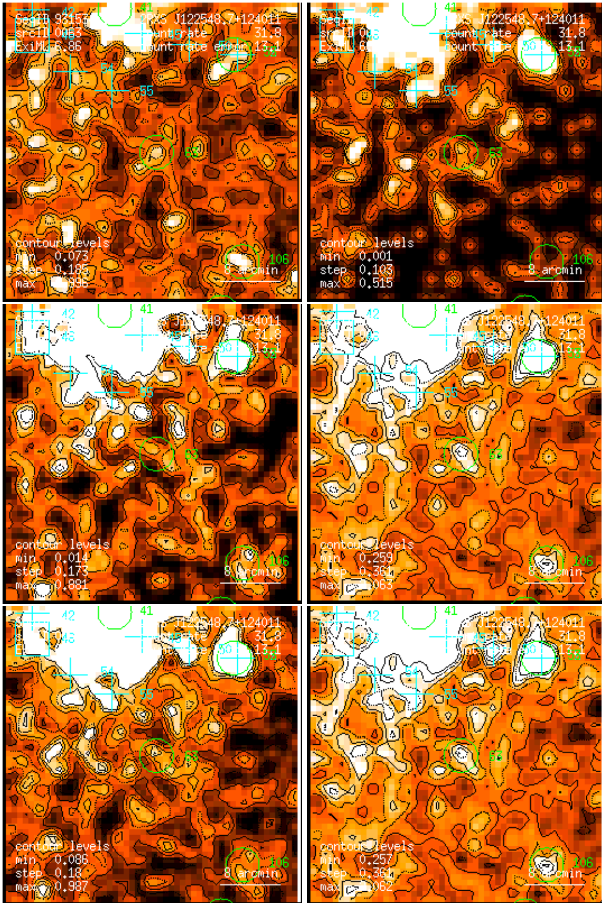
Figure 63: RASS 931534: detection 0063: band rate images, Gaussian filter: (1) PSPC channels 11 – 41, (2) 52 – 90, (3) 91 – 201, (4) 11 – 235, (5) 52 – 201, (6) 11 – 201. Broad band rates in counts/ks. Band rate contour levels in counts/ks/arcmin 2 .
