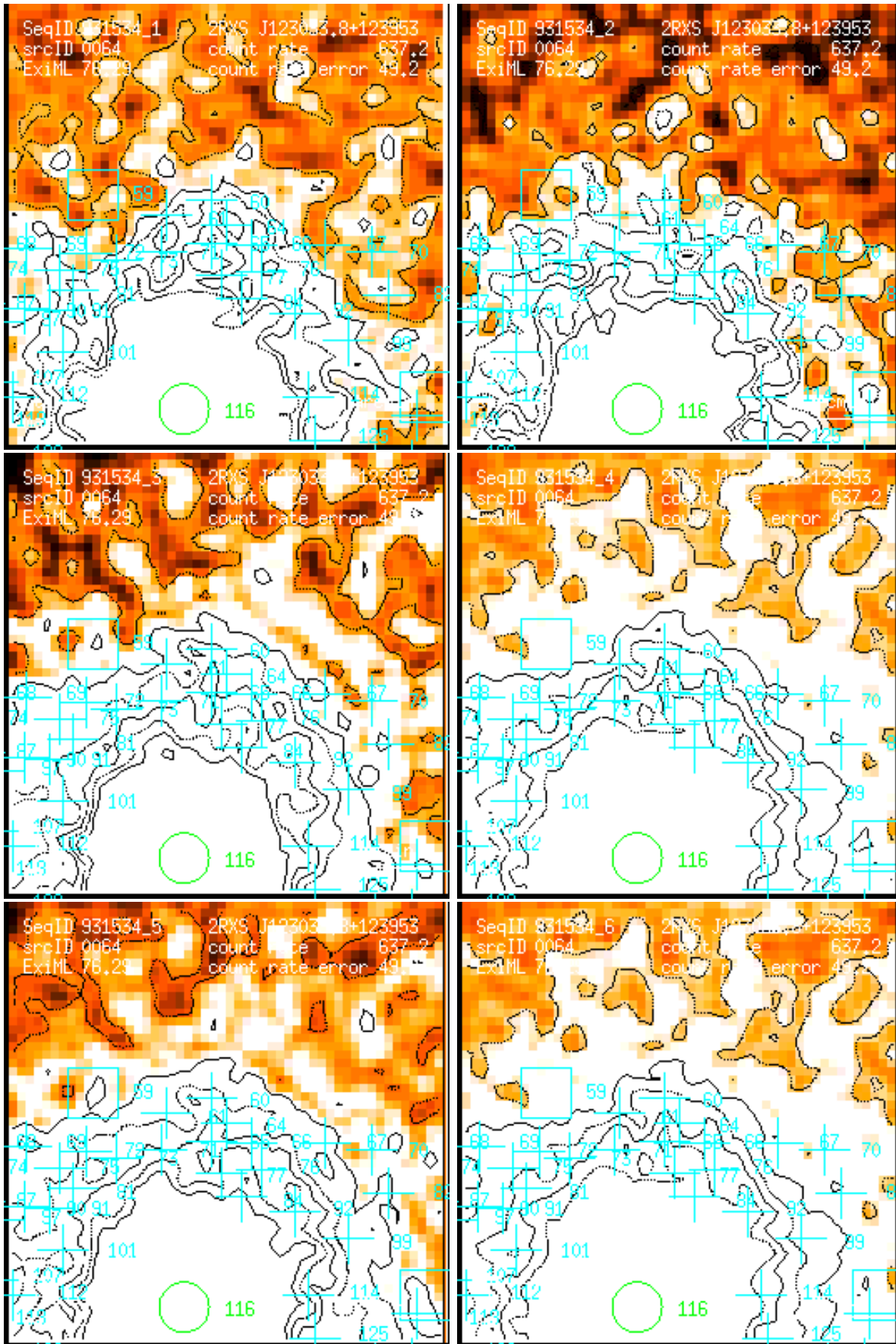
Figure 64: RASS 931534: detection 0064: band rate images, Gaussian filter: (1) PSPC channels 11 – 41, (2) 52 – 90, (3) 91 – 201, (4) 11 – 235, (5) 52 – 201, (6) 11 – 201. Broad band rates in counts/ks. Band rate contour levels in counts/ks/arcmin 2 .
