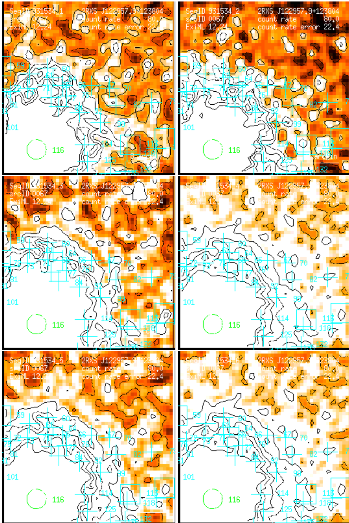
Figure 67: RASS 931534: detection 0067: band rate images, Gaussian filter: (1) PSPC channels 11 – 41, (2) 52 – 90, (3) 91 – 201, (4) 11 – 235, (5) 52 – 201, (6) 11 – 201. Broad band rates in counts/ks. Band rate contour levels in counts/ks/arcmin 2 .
