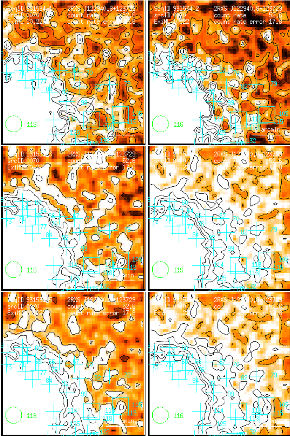
Figure 70: RASS 931534: detection 0070: band rate images, Gaussian filter: (1) PSPC channels 11 – 41, (2) 52 – 90, (3) 91 – 201, (4) 11 – 235, (5) 52 – 201, (6) 11 – 201. Broad band rates in counts/ks. Band rate contour levels in counts/ks/arcmin 2 .
