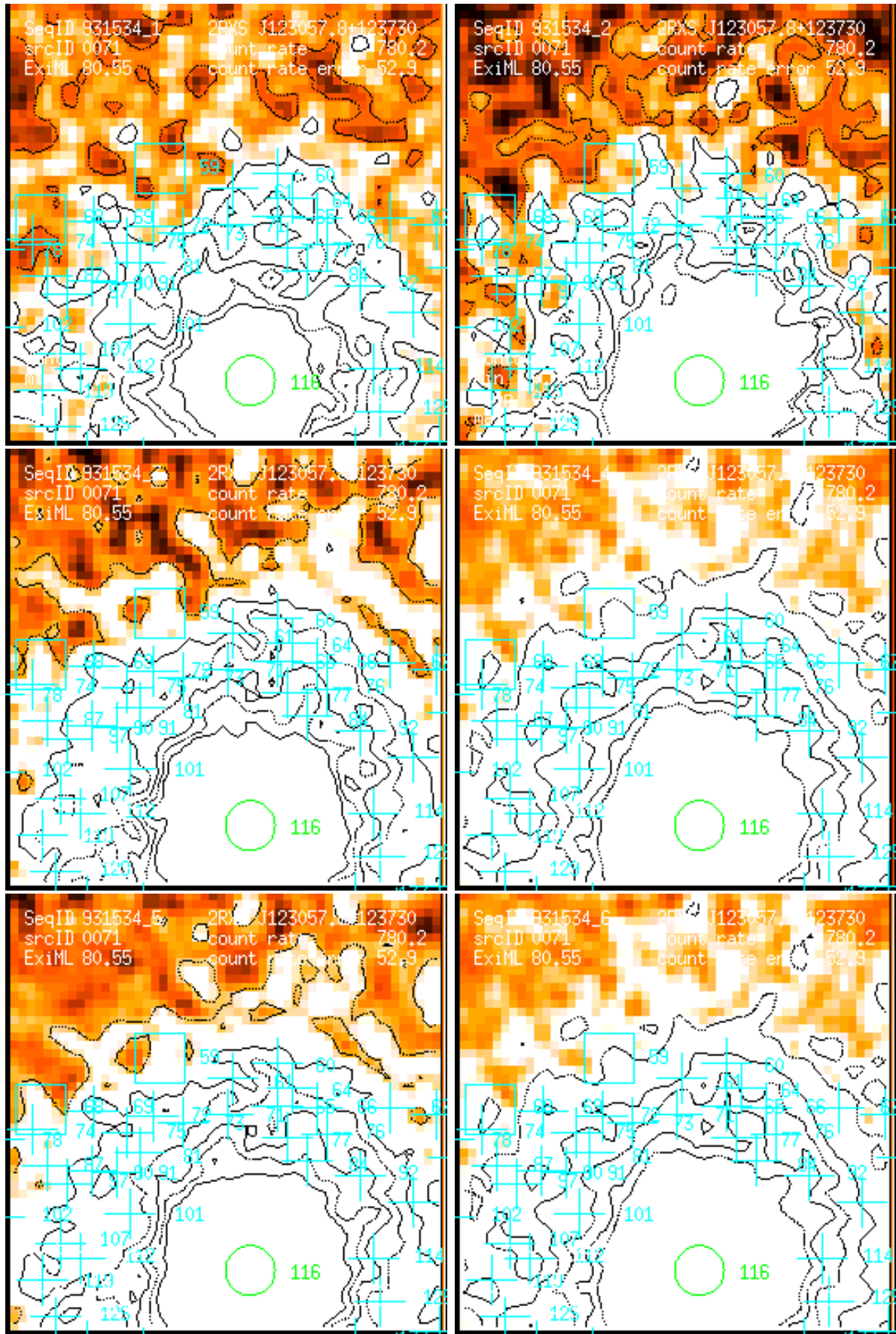
Figure 71: RASS 931534: detection 0071: band rate images, Gaussian filter: (1) PSPC channels 11 – 41, (2) 52 – 90, (3) 91 – 201, (4) 11 – 235, (5) 52 – 201, (6) 11 – 201. Broad band rates in counts/ks. Band rate contour levels in counts/ks/arcmin 2 .
