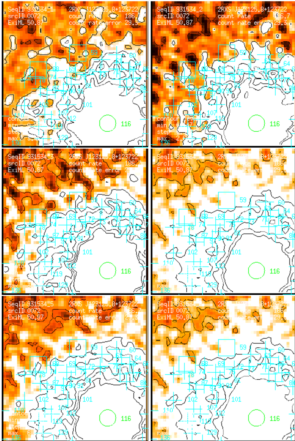
Figure 72: RASS 931534: detection 0072: band rate images, Gaussian filter: (1) PSPC channels 11 – 41, (2) 52 – 90, (3) 91 – 201, (4) 11 – 235, (5) 52 – 201, (6) 11 – 201. Broad band rates in counts/ks. Band rate contour levels in counts/ks/arcmin 2 .
