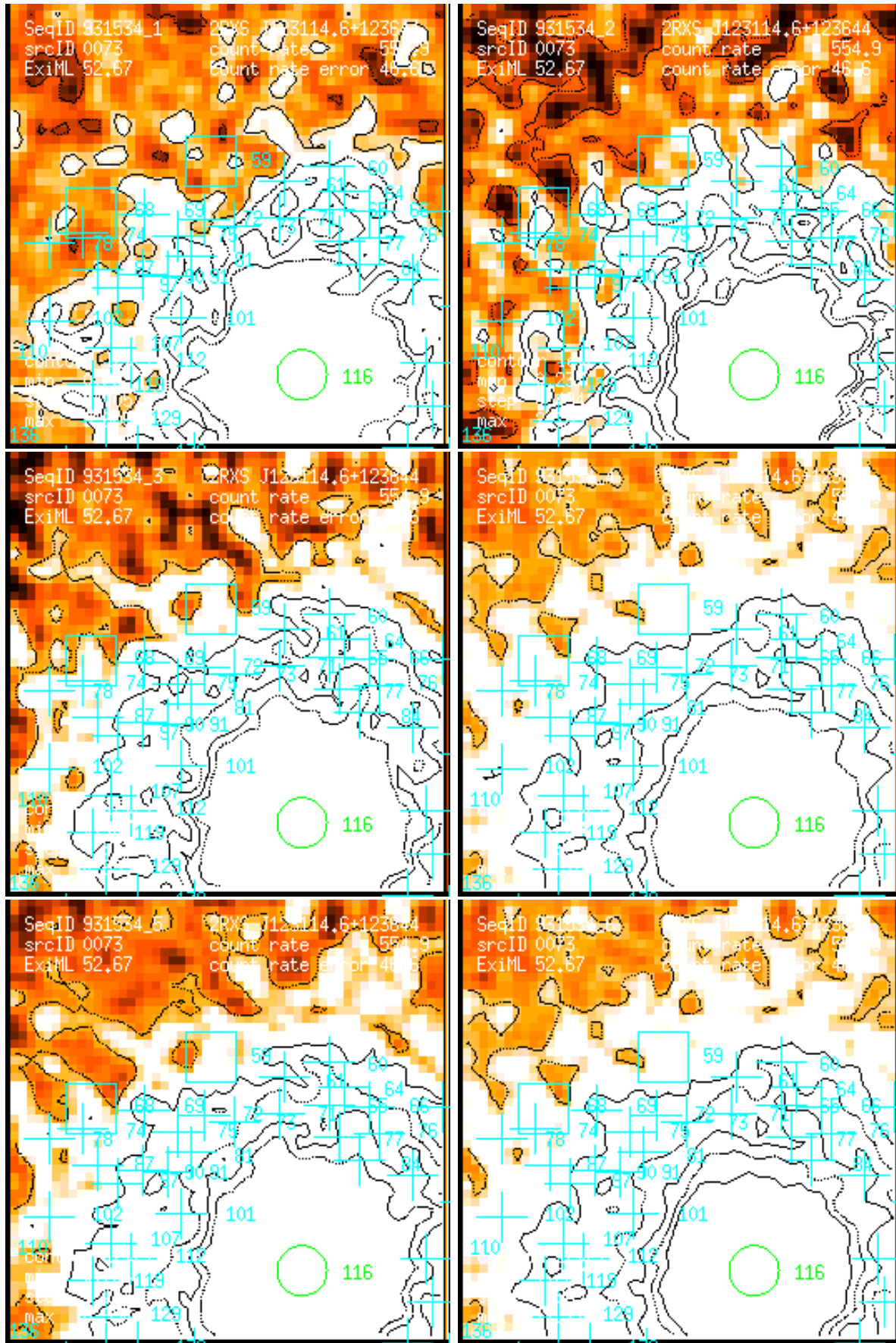
Figure 73: RASS 931534: detection 0073: band rate images, Gaussian filter: (1) PSPC channels 11 – 41, (2) 52 – 90, (3) 91 – 201, (4) 11 – 235, (5) 52 – 201, (6) 11 – 201. Broad band rates in counts/ks. Band rate contour levels in counts/ks/arcmin 2 .
