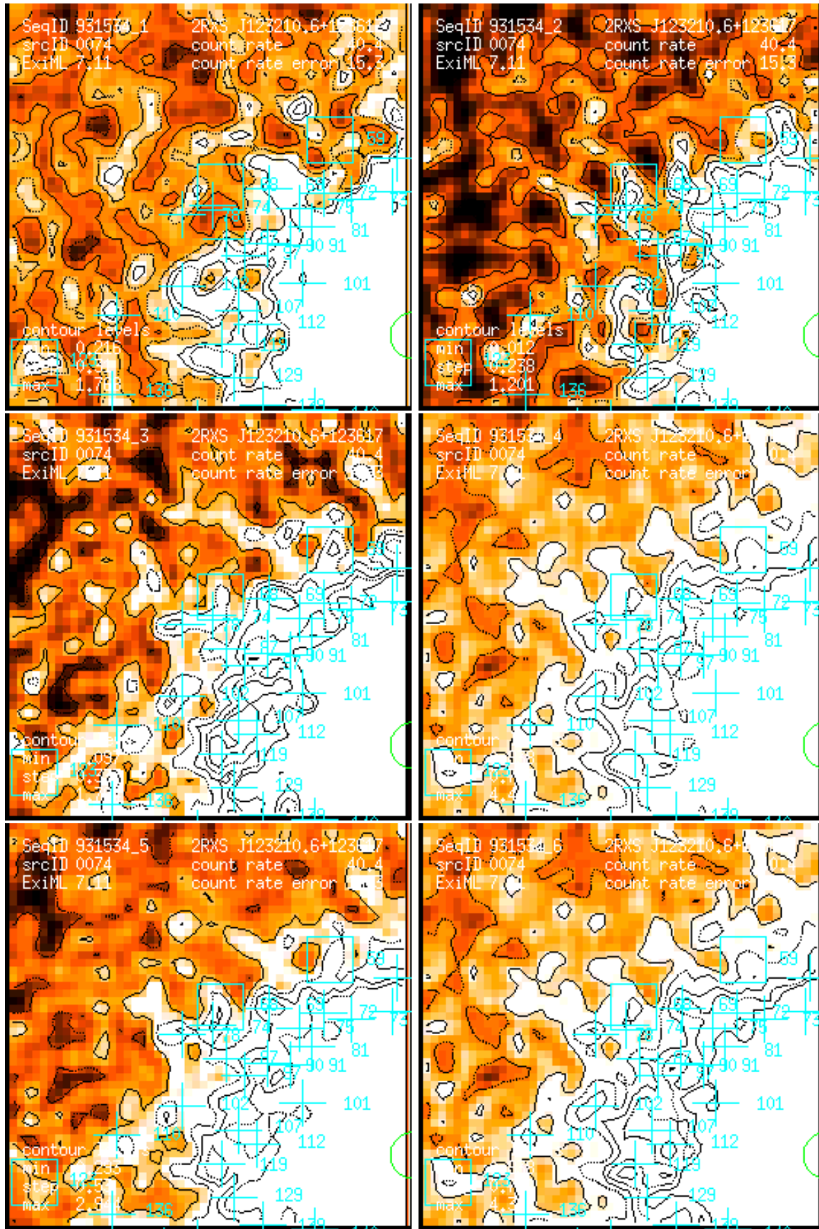
Figure 74: RASS 931534: detection 0074: band rate images, Gaussian filter: (1) PSPC channels 11 – 41, (2) 52 – 90, (3) 91 – 201, (4) 11 – 235, (5) 52 – 201, (6) 11 – 201. Broad band rates in counts/ks. Band rate contour levels in counts/ks/arcmin 2 .
