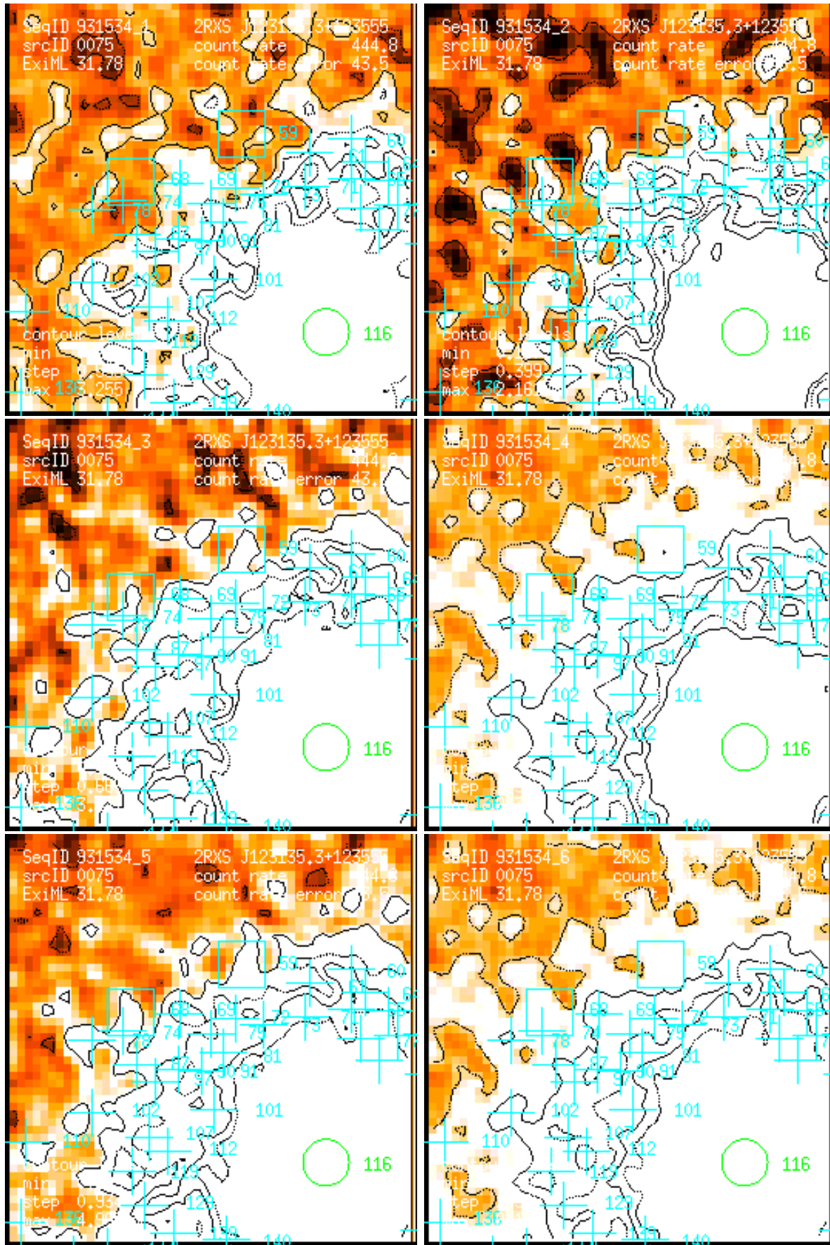
Figure 75: RASS 931534: detection 0075: band rate images, Gaussian filter: (1) PSPC channels 11 – 41, (2) 52 – 90, (3) 91 – 201, (4) 11 – 235, (5) 52 – 201, (6) 11 – 201. Broad band rates in counts/ks. Band rate contour levels in counts/ks/arcmin 2 .
