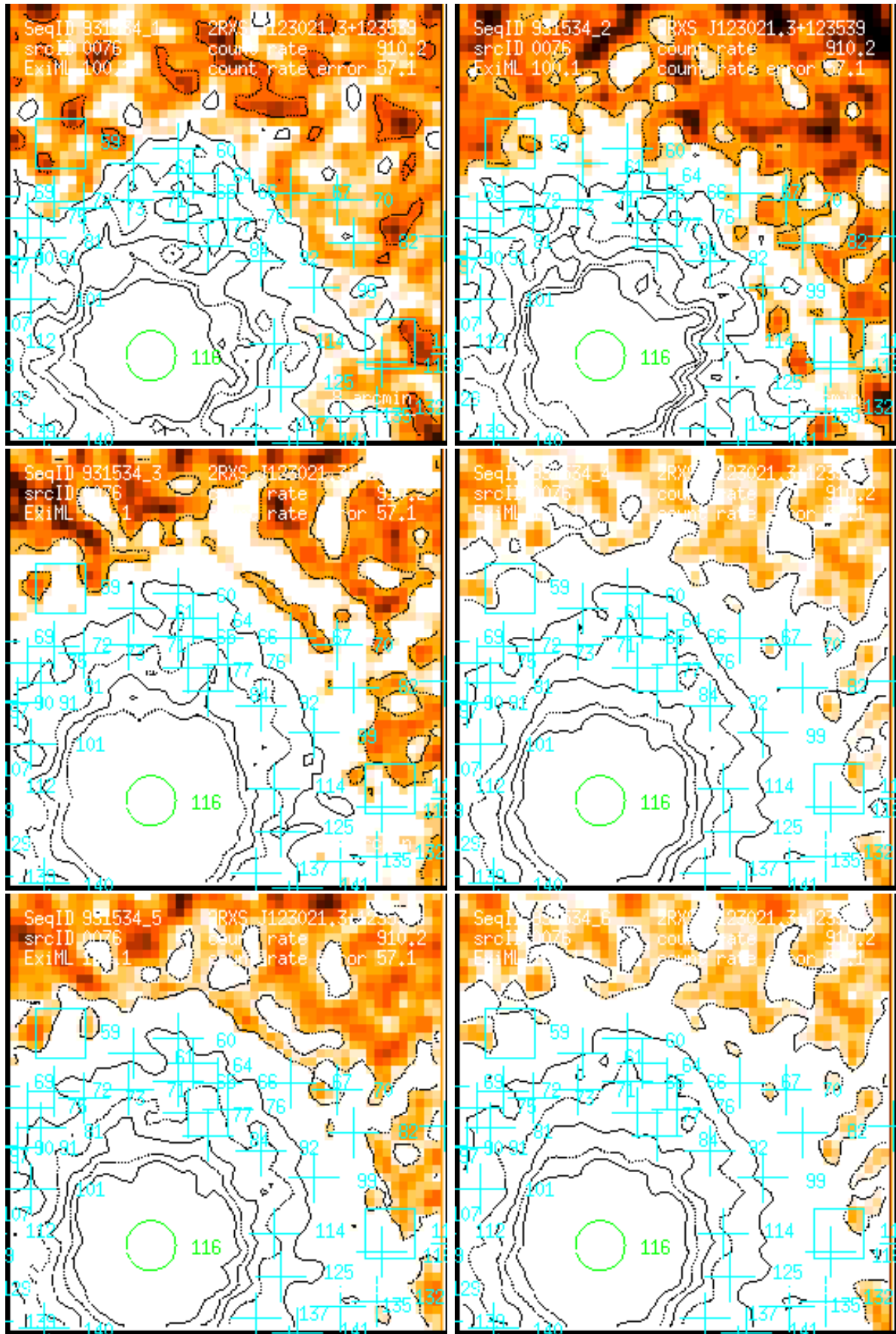
Figure 76: RASS 931534: detection 0076: band rate images, Gaussian filter: (1) PSPC channels 11 – 41, (2) 52 – 90, (3) 91 – 201, (4) 11 – 235, (5) 52 – 201, (6) 11 – 201. Broad band rates in counts/ks. Band rate contour levels in counts/ks/arcmin 2 .
