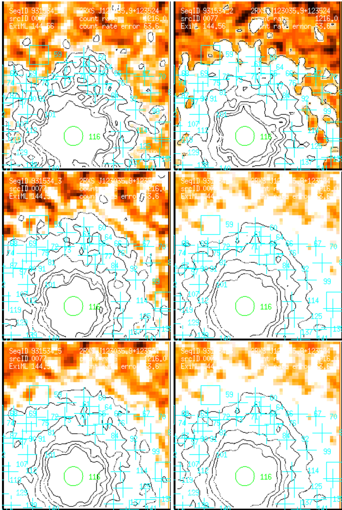
Figure 77: RASS 931534: detection 0077: band rate images, Gaussian filter: (1) PSPC channels 11 – 41, (2) 52 – 90, (3) 91 – 201, (4) 11 – 235, (5) 52 – 201, (6) 11 – 201. Broad band rates in counts/ks. Band rate contour levels in counts/ks/arcmin 2 .
