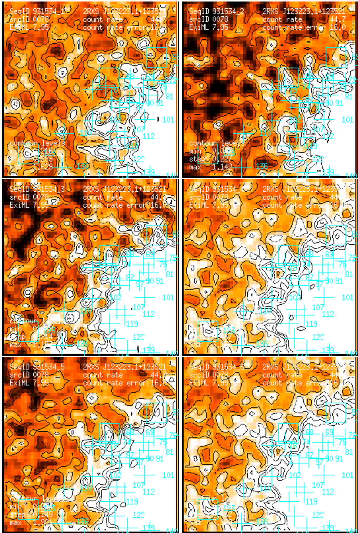
Figure 78: RASS 931534: detection 0078: band rate images, Gaussian filter: (1) PSPC channels 11 – 41, (2) 52 – 90, (3) 91 – 201, (4) 11 – 235, (5) 52 – 201, (6) 11 – 201. Broad band rates in counts/ks. Band rate contour levels in counts/ks/arcmin 2 .
