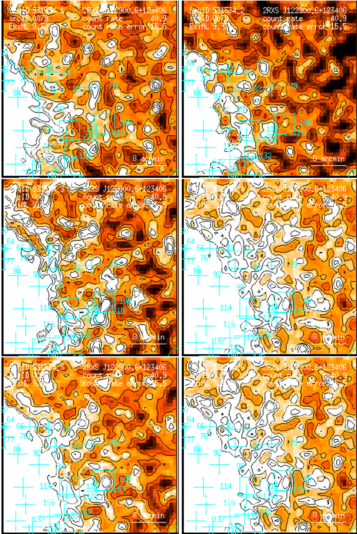
Figure 79: RASS 931534: detection 0079: band rate images, Gaussian filter: (1) PSPC channels 11 – 41, (2) 52 – 90, (3) 91 – 201, (4) 11 – 235, (5) 52 – 201, (6) 11 – 201. Broad band rates in counts/ks. Band rate contour levels in counts/ks/arcmin 2 .
