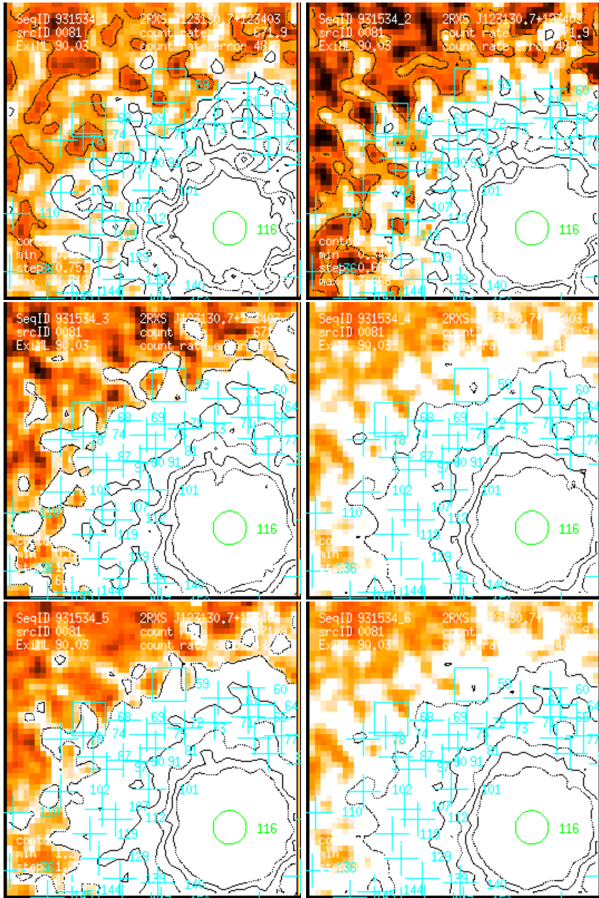
Figure 81: RASS 931534: detection 0081: band rate images, Gaussian filter: (1) PSPC channels 11 – 41, (2) 52 – 90, (3) 91 – 201, (4) 11 – 235, (5) 52 – 201, (6) 11 – 201. Broad band rates in counts/ks. Band rate contour levels in counts/ks/arcmin 2 .
