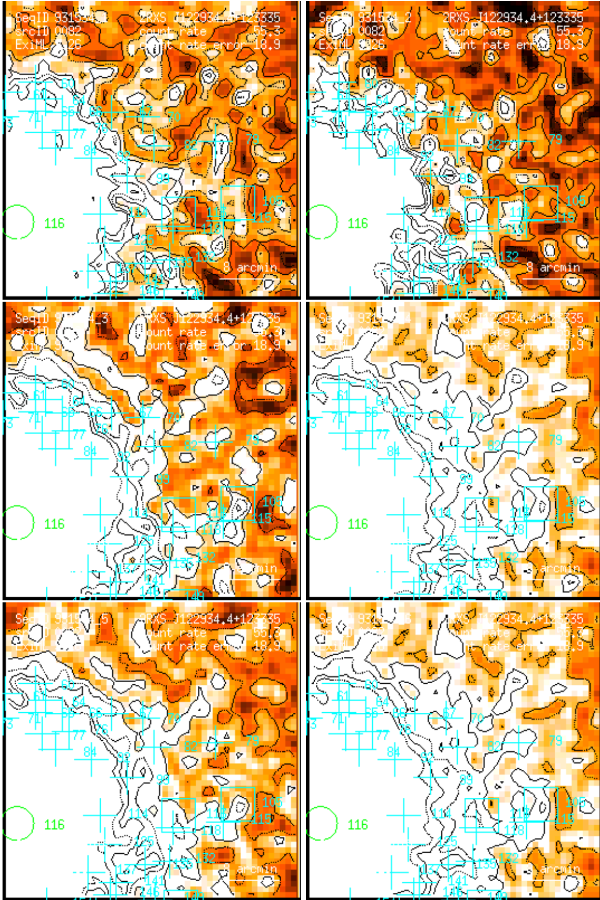
Figure 82: RASS 931534: detection 0082: band rate images, Gaussian filter: (1) PSPC channels 11 – 41, (2) 52 – 90, (3) 91 – 201, (4) 11 – 235, (5) 52 – 201, (6) 11 – 201. Broad band rates in counts/ks. Band rate contour levels in counts/ks/arcmin 2 .
