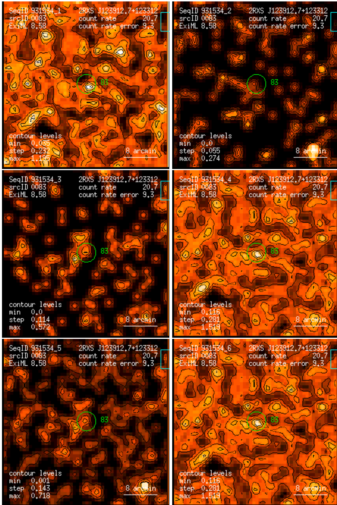
Figure 83: RASS 931534: detection 0083: band rate images, Gaussian filter: (1) PSPC channels 11 – 41, (2) 52 – 90, (3) 91 – 201, (4) 11 – 235, (5) 52 – 201, (6) 11 – 201. Broad band rates in counts/ks. Band rate contour levels in counts/ks/arcmin 2 .
