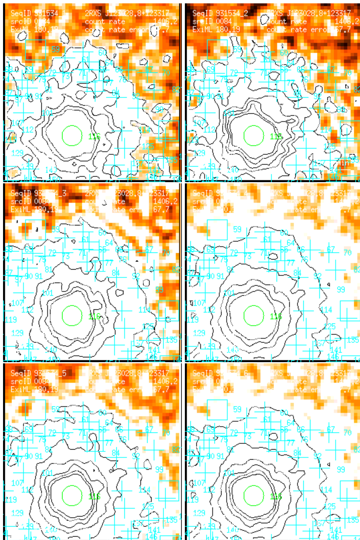
Figure 84: RASS 931534: detection 0084: band rate images, Gaussian filter: (1) PSPC channels 11 – 41, (2) 52 – 90, (3) 91 – 201, (4) 11 – 235, (5) 52 – 201, (6) 11 – 201. Broad band rates in counts/ks. Band rate contour levels in counts/ks/arcmin 2 .
