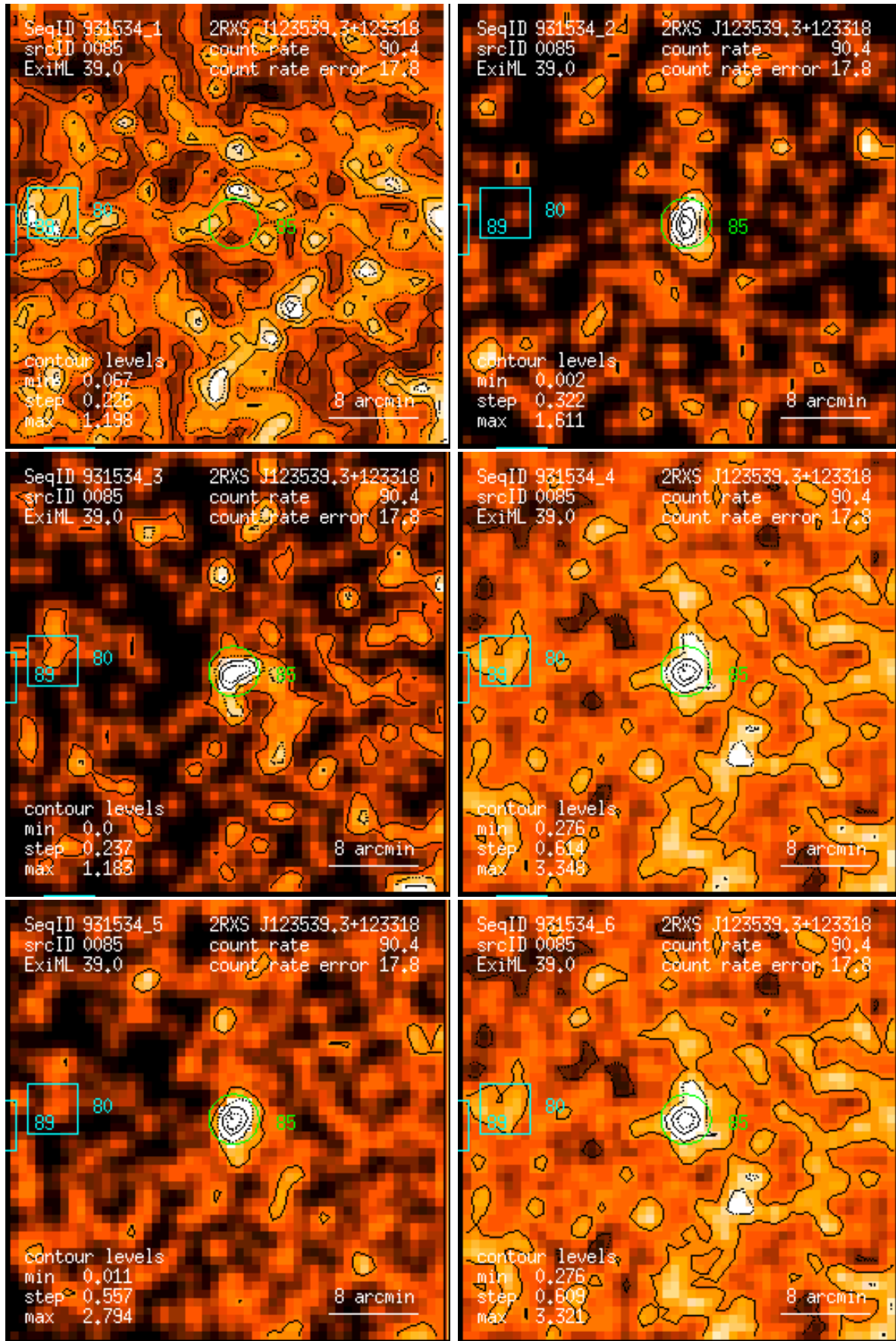
Figure 85: RASS 931534: detection 0085: band rate images, Gaussian filter: (1) PSPC channels 11 – 41, (2) 52 – 90, (3) 91 – 201, (4) 11 – 235, (5) 52 – 201, (6) 11 – 201. Broad band rates in counts/ks. Band rate contour levels in counts/ks/arcmin 2 .
