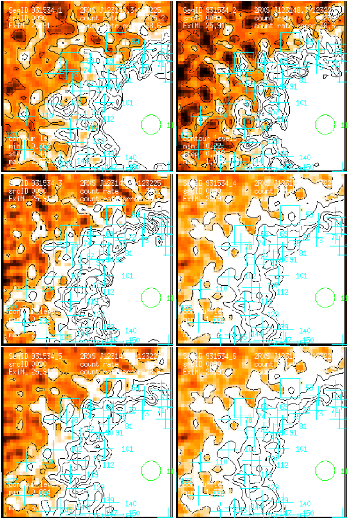
Figure 90: RASS 931534: detection 0090: band rate images, Gaussian filter: (1) PSPC channels 11 – 41, (2) 52 – 90, (3) 91 – 201, (4) 11 – 235, (5) 52 – 201, (6) 11 – 201. Broad band rates in counts/ks. Band rate contour levels in counts/ks/arcmin 2 .
