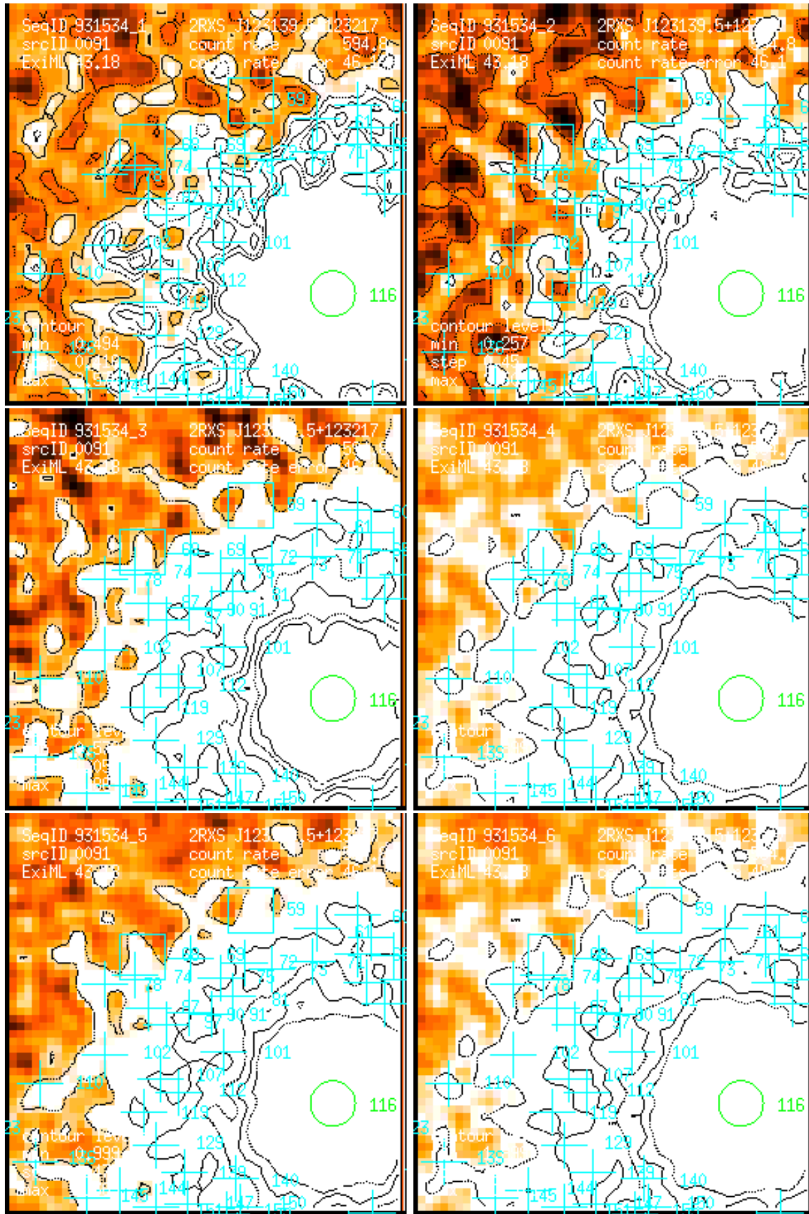
Figure 91: RASS 931534: detection 0091: band rate images, Gaussian filter: (1) PSPC channels 11 – 41, (2) 52 – 90, (3) 91 – 201, (4) 11 – 235, (5) 52 – 201, (6) 11 – 201. Broad band rates in counts/ks. Band rate contour levels in counts/ks/arcmin 2 .
