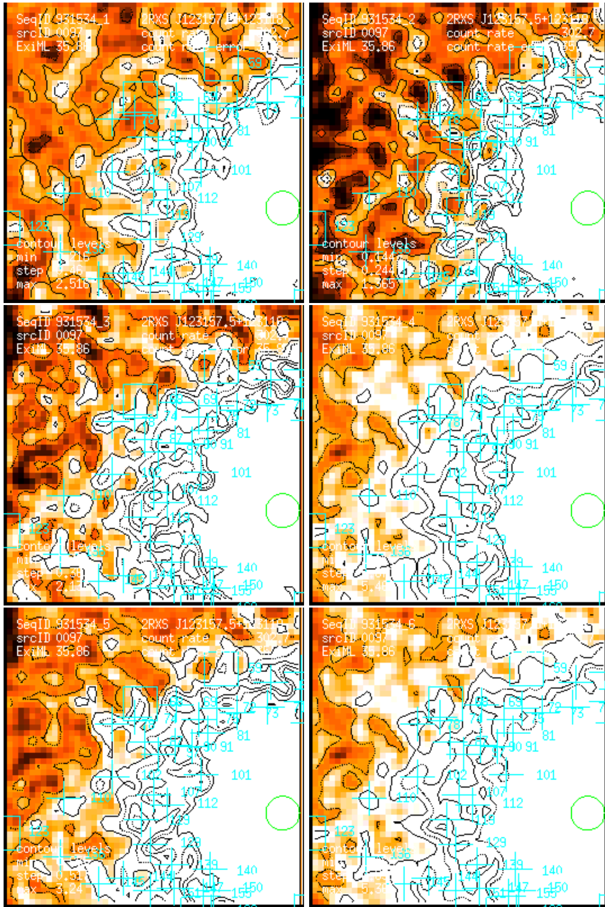
Figure 97: RASS 931534: detection 0097: band rate images, Gaussian filter: (1) PSPC channels 11 – 41, (2) 52 – 90, (3) 91 – 201, (4) 11 – 235, (5) 52 – 201, (6) 11 – 201. Broad band rates in counts/ks. Band rate contour levels in counts/ks/arcmin 2 .
