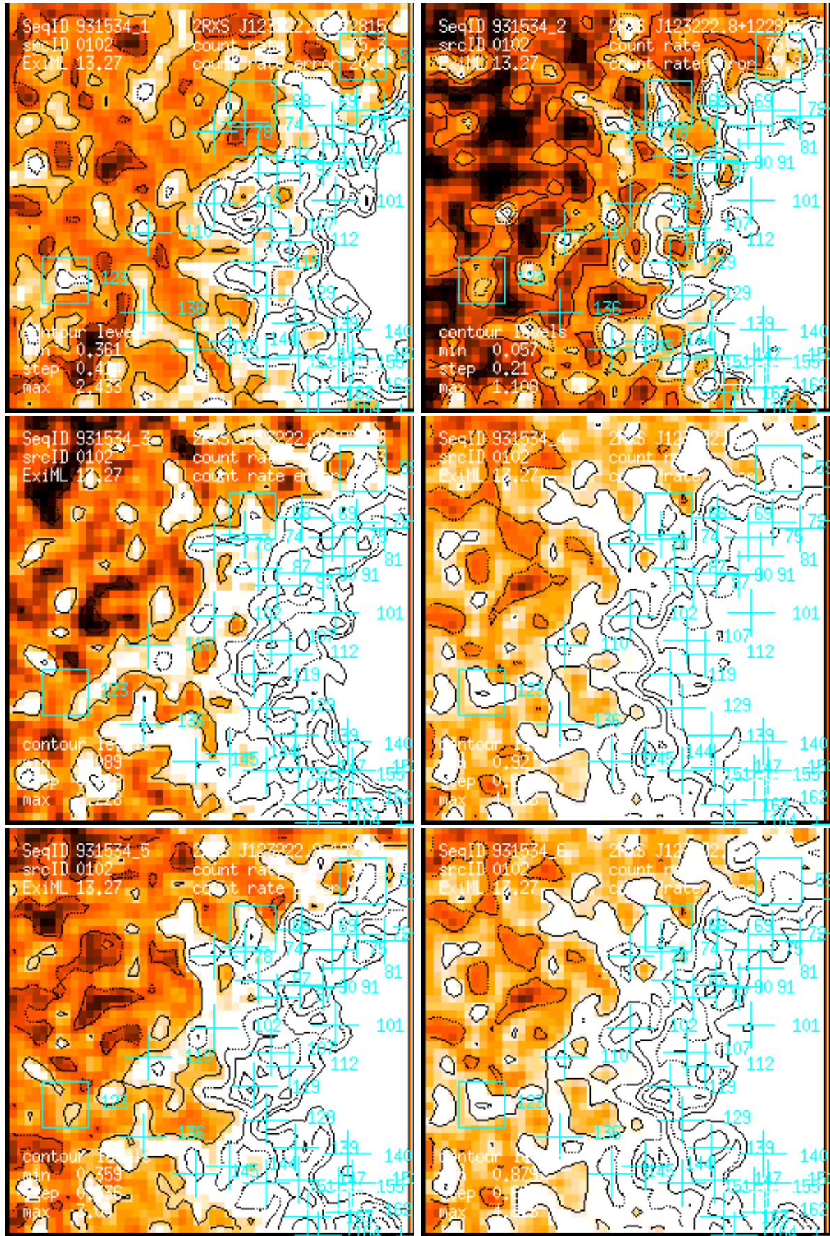
Figure 102: RASS 931534: detection 0102: band rate images, Gaussian filter: (1) PSPC channels 11 – 41, (2) 52 – 90, (3) 91 – 201, (4) 11 – 235, (5) 52 – 201, (6) 11 – 201. Broad band rates in counts/ks. Band rate contour levels in counts/ks/arcmin 2 .
