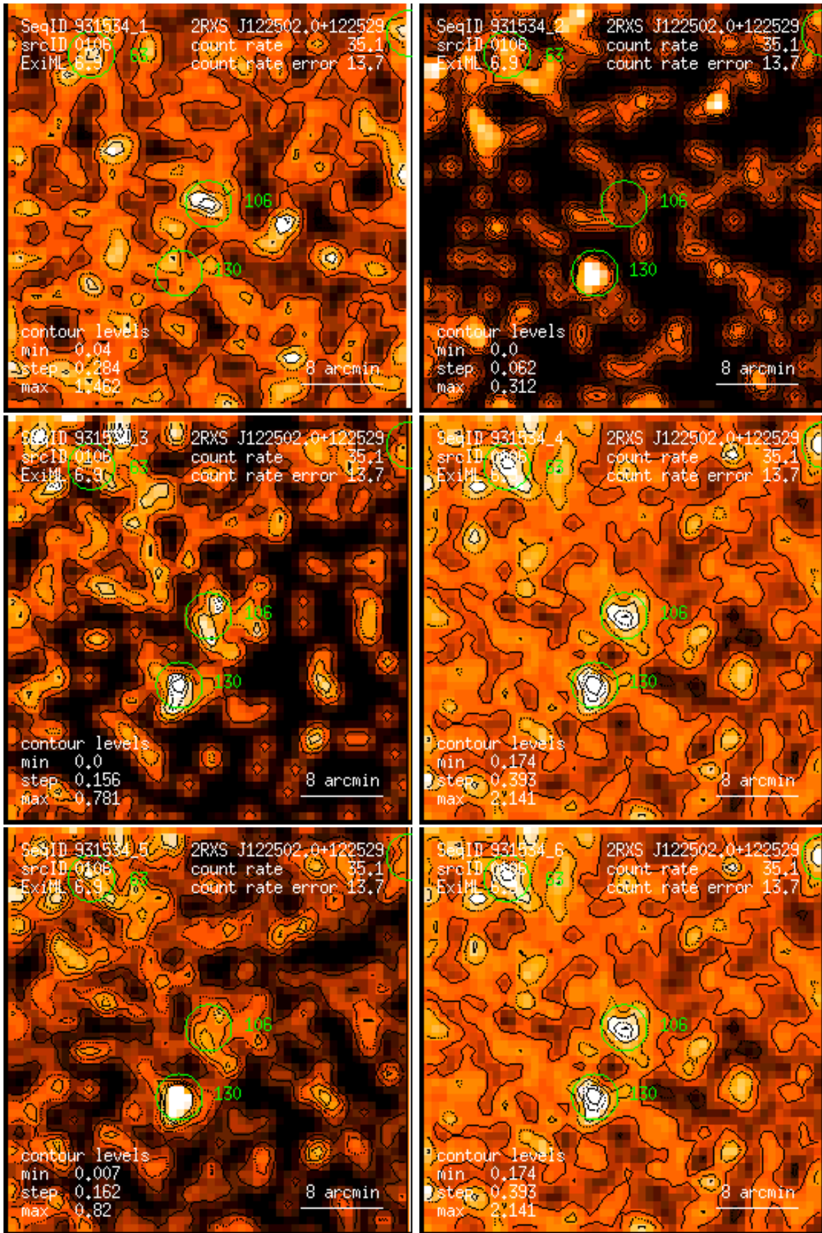
Figure 106: RASS 931534: detection 0106: band rate images, Gaussian filter: (1) PSPC channels 11 – 41, (2) 52 – 90, (3) 91 – 201, (4) 11 – 235, (5) 52 – 201, (6) 11 – 201. Broad band rates in counts/ks. Band rate contour levels in counts/ks/arcmin 2 .
