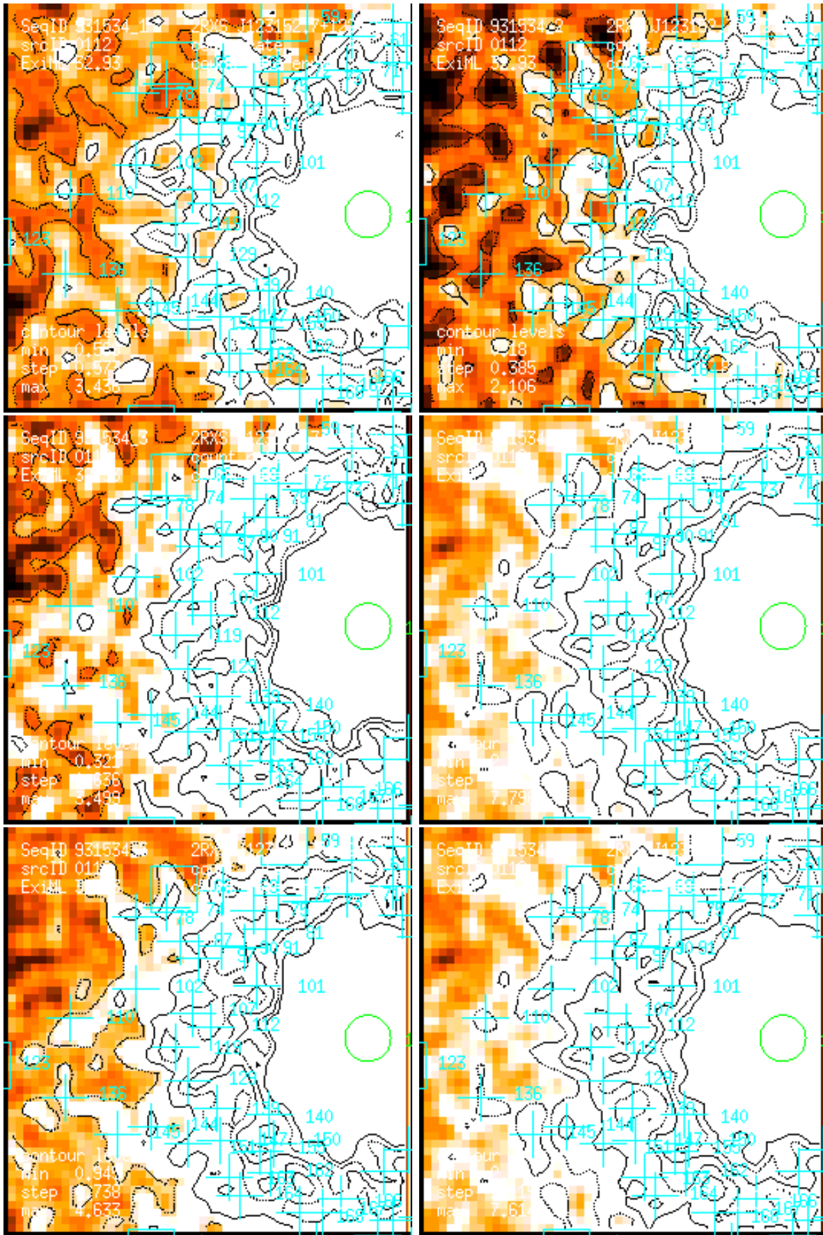
Figure 112: RASS 931534: detection 0112: band rate images, Gaussian filter: (1) PSPC channels 11 – 41, (2) 52 – 90, (3) 91 – 201, (4) 11 – 235, (5) 52 – 201, (6) 11 – 201. Broad band rates in counts/ks. Band rate contour levels in counts/ks/arcmin 2 .
