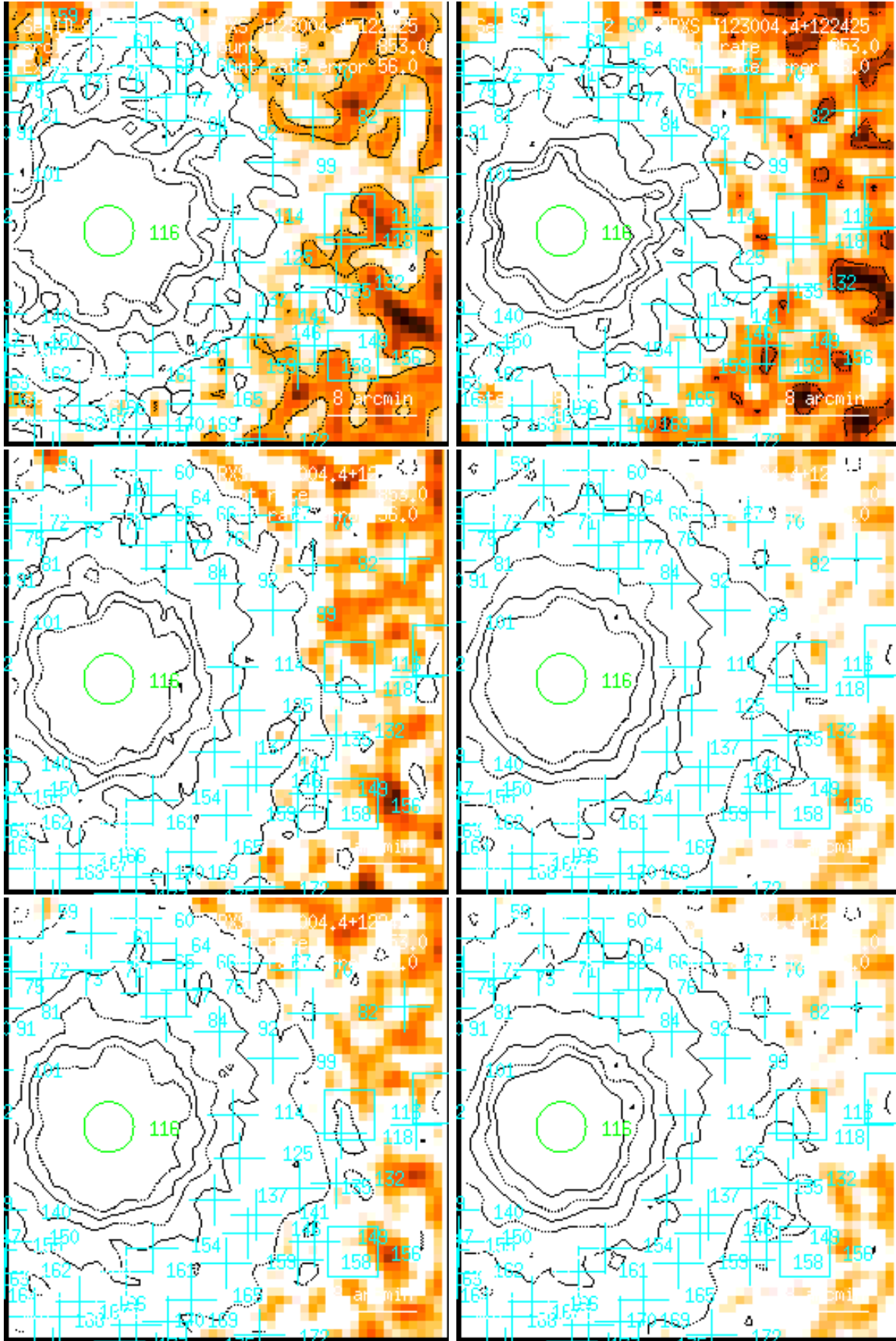
Figure 114: RASS 931534: detection 0114: band rate images, Gaussian filter: (1) PSPC channels 11 – 41, (2) 52 – 90, (3) 91 – 201, (4) 11 – 235, (5) 52 – 201, (6) 11 – 201. Broad band rates in counts/ks. Band rate contour levels in counts/ks/arcmin 2 .
