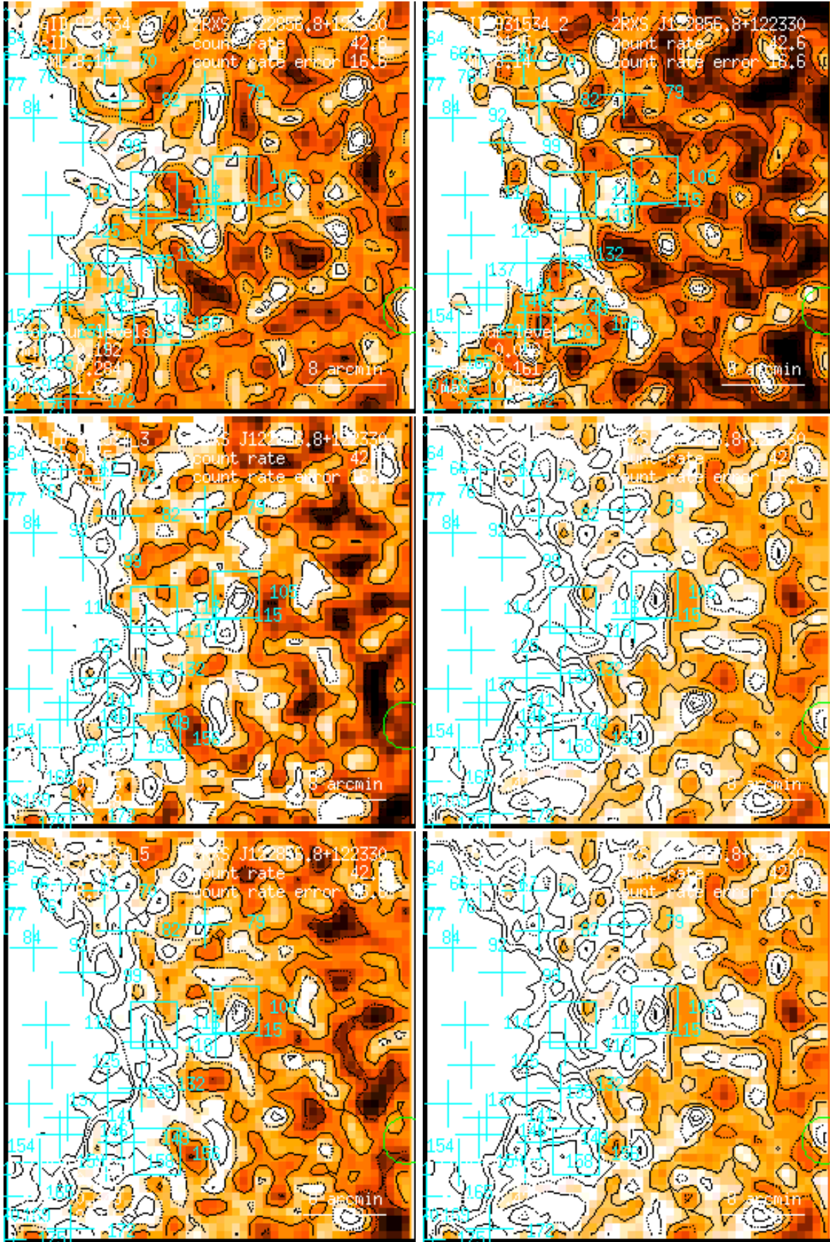
Figure 115: RASS 931534: detection 0115: band rate images, Gaussian filter: (1) PSPC channels 11 – 41, (2) 52 – 90, (3) 91 – 201, (4) 11 – 235, (5) 52 – 201, (6) 11 – 201. Broad band rates in counts/ks. Band rate contour levels in counts/ks/arcmin 2 .
