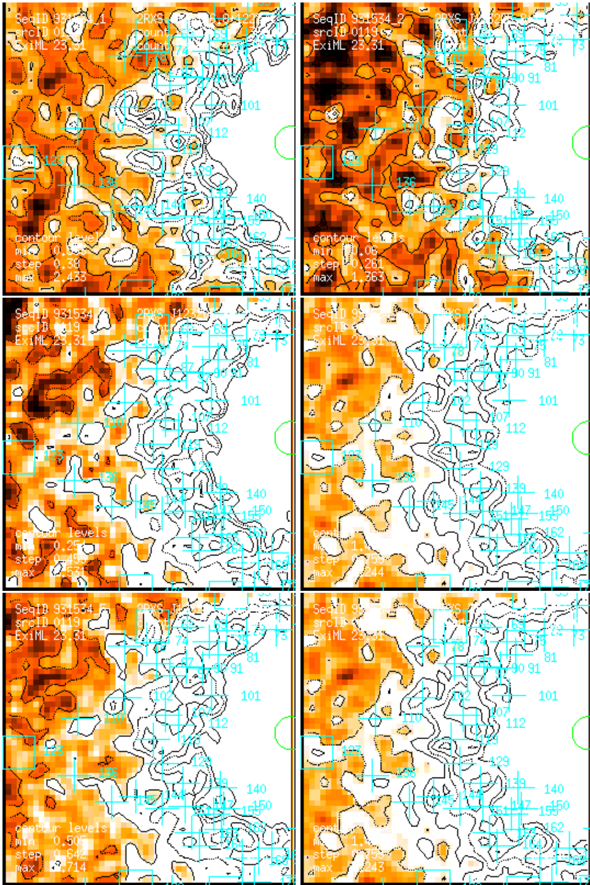
Figure 119: RASS 931534: detection 0119: band rate images, Gaussian filter: (1) PSPC channels 11 – 41, (2) 52 – 90, (3) 91 – 201, (4) 11 – 235, (5) 52 – 201, (6) 11 – 201. Broad band rates in counts/ks. Band rate contour levels in counts/ks/arcmin 2 .
